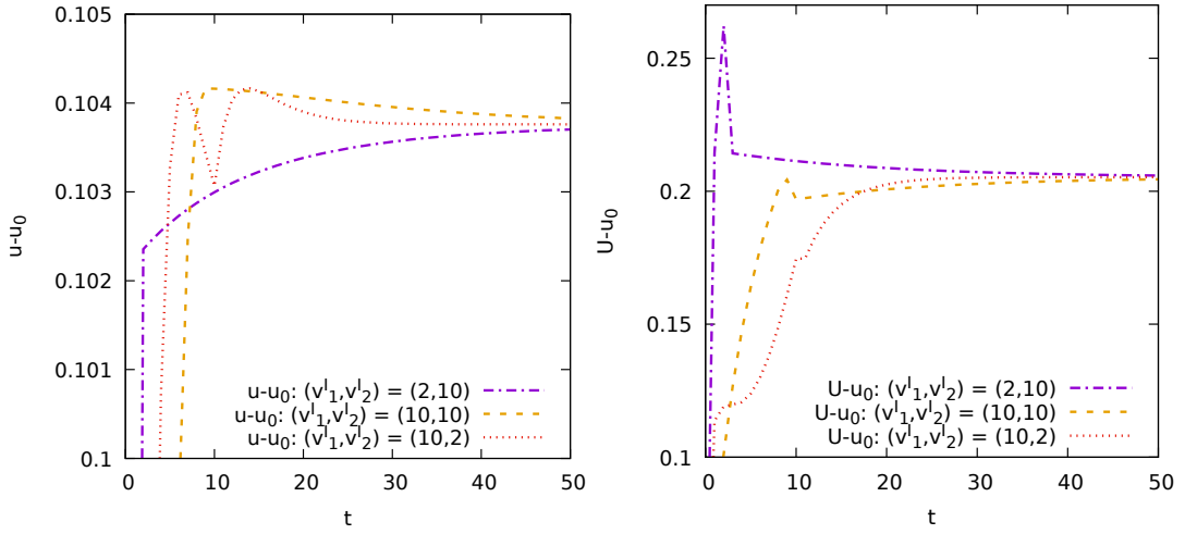
Figure 13: Total intrinsic utility u (left) and total utility U (right), relative to utility without consumption ( u_0 = w_1 + w_2 ); case [bII.1] with excess then shortage; varying v_1^I
