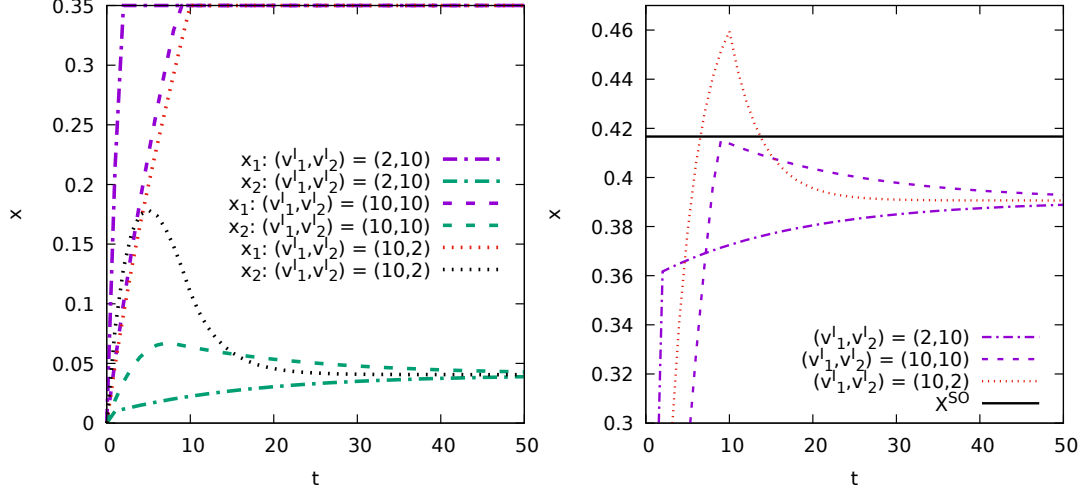
Figure 12: Individual (left) and total (right) contributions; case [bII.1] with excess then shortage; varying v_1^I
