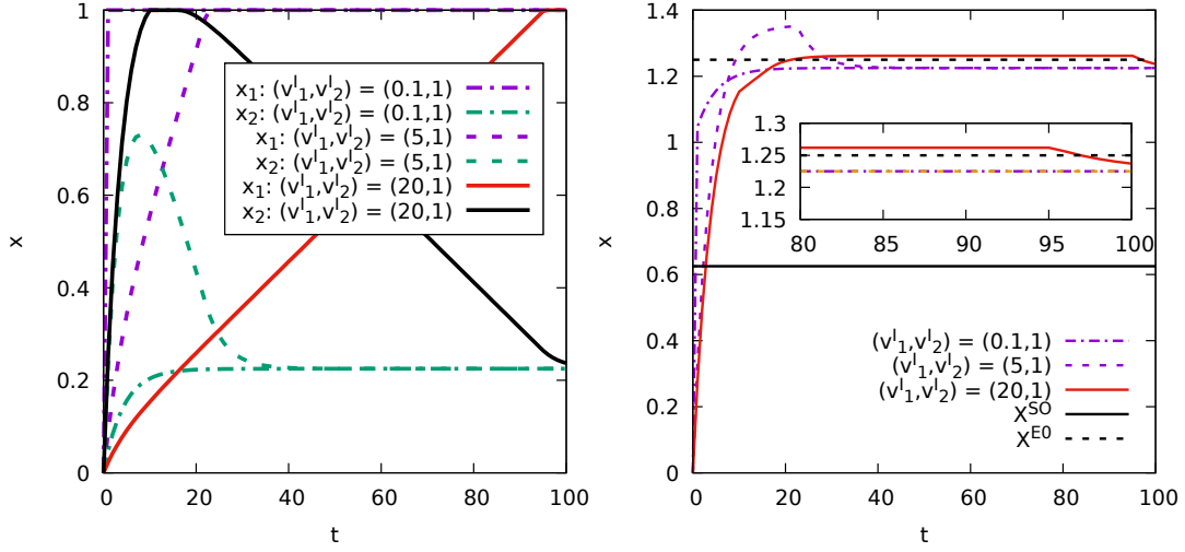
Figure 10: Individual (left) and total (right) contributions; case [bII.1] with welfare reduction then shortage; varying v_1^I
