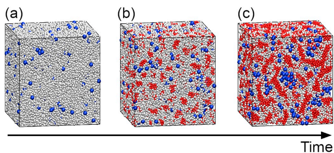
Fig. 6. Snapshots from coarse-grain MD simulations of enzymes acting on polymers modelled as chains of monomers. The enzymes (blue spheres) are able to convert initially repulsive monomers (white spheres) into attractive monomers (red spheres). The initially homogeneous system (a) forms clusters of attractive monomers at an intermediate stage (b) and eventually turns into a gel (c). The simulation box contains 400 polymers of 100 monomers and 500 enzymes, corresponding to a total volume fraction of 30%. (For interpretation of the references to color in this figure legend, the reader is referred to the web version of this article.)
