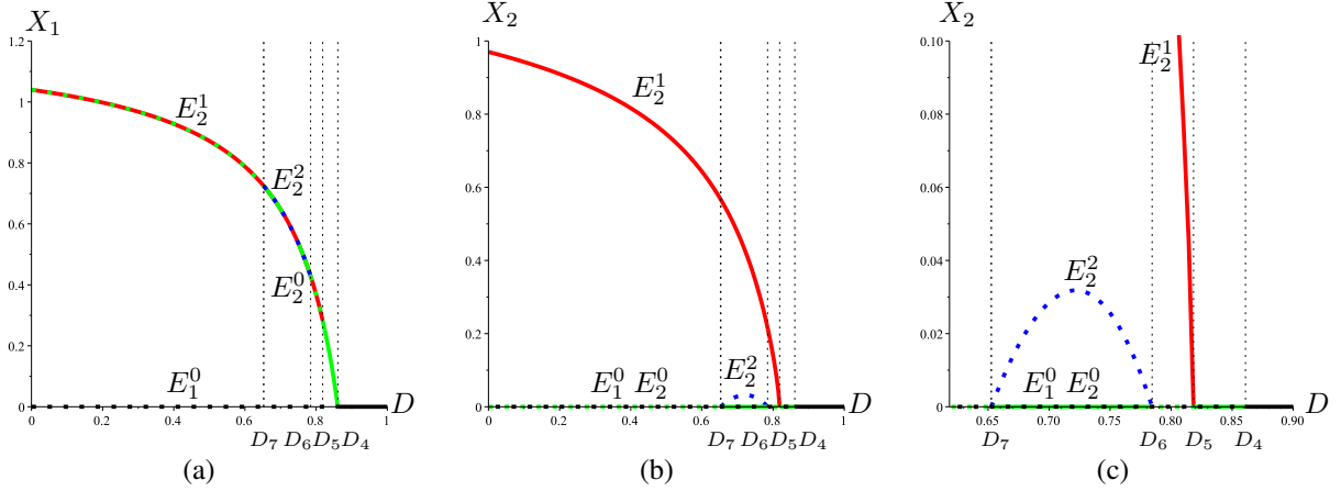
Figure 11: Bifurcation diagram with D as the bifurcation parameter, corresponding to Fig. 7(a) and S_{lin} = 13 . (a): The X_1 -components and (b): the X_2 -components, of the steady states E_1^0 (in Black), E_2^0 (in Green), E_2^1 (in Red) and E_2^2 (in Blue). (c): A magnification showing the bifurcation values D_4 , D_5 , D_6 and D_7 . Solid lines and dotted lines correspond to stable and unstable steady states respectively.
