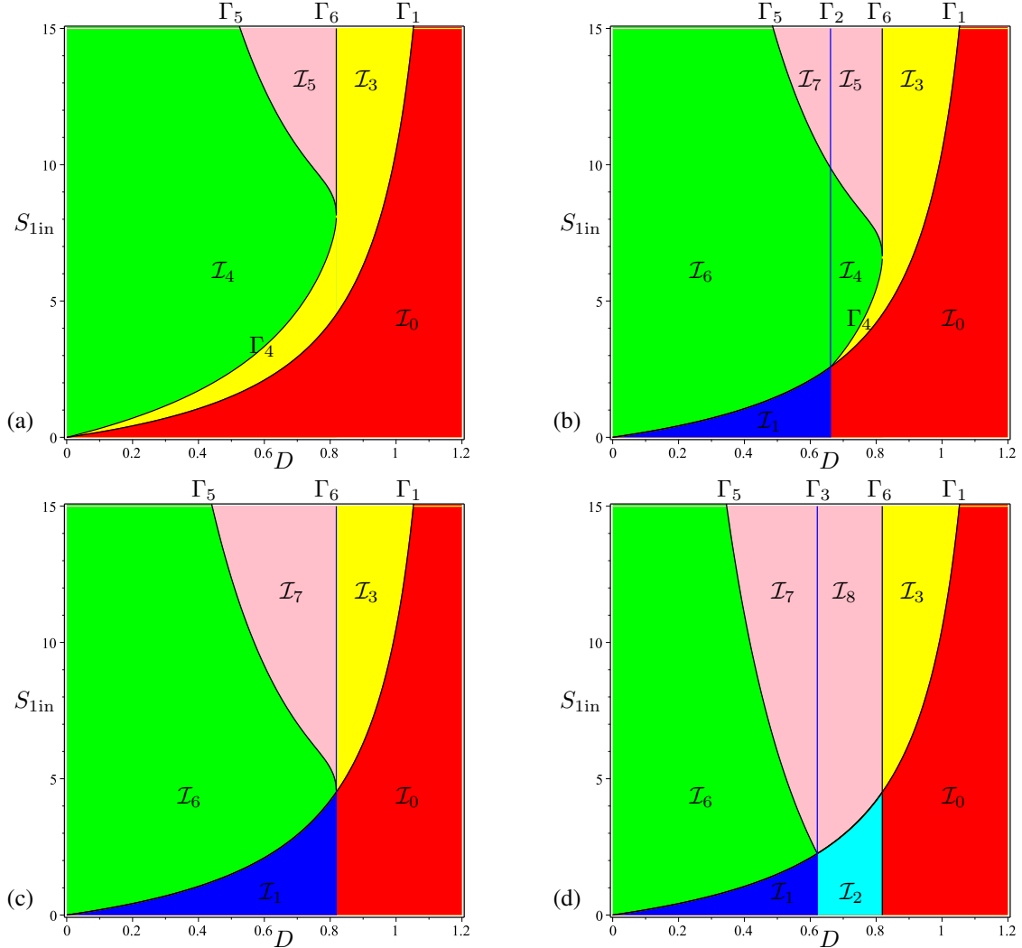
Figure 6: The 2-dimensional operating diagram (D, S_{1in}) obtained by cuts at S_{2in} constant of the 3-dimensional operating diagram shown in Fig. 2 and corresponding to Fig. 1(a). (a): S_{2in} = 0 , (b): S_{2in} = 15 , (c): S_{2in} = S_2^M \simeq 36.332 and (d): S_{2in} = 100 .
