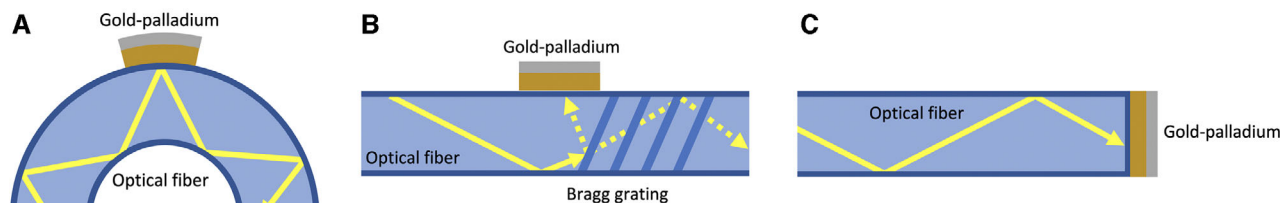
FIGURE 4 Optical fiber configurations. Optical fibers with a gold-palladium layer stack showing configurations that can increase the angle of the light incident with the fiber surface. A D-loop consists of a 180° bend in an optical fiber that results in a higher angle for light interacting with the fiber surface on the outside of the bend (A). Optical fiber Bragg gratings are etched into the core of the fiber, directing light toward the surface of the fiber at the desired angle (B). An endcap allows incident light to interact with a surface at a high incident angle (C)
