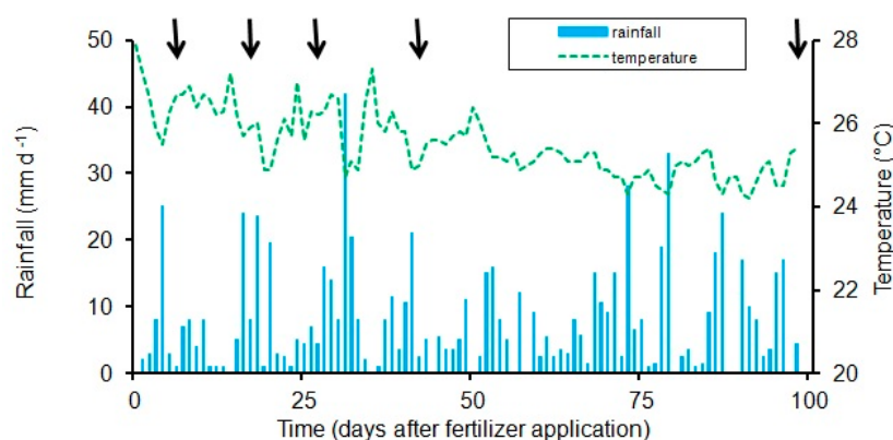
Figure 2. Rainfall and air temperature after the application of the ^{15}\text{N} fertilizer at flowering (10 October 2004, Day 0). Arrows indicate the dates of soil sampling. The last soil sampling was carried out at harvest (16 January 2005, Day 98).
