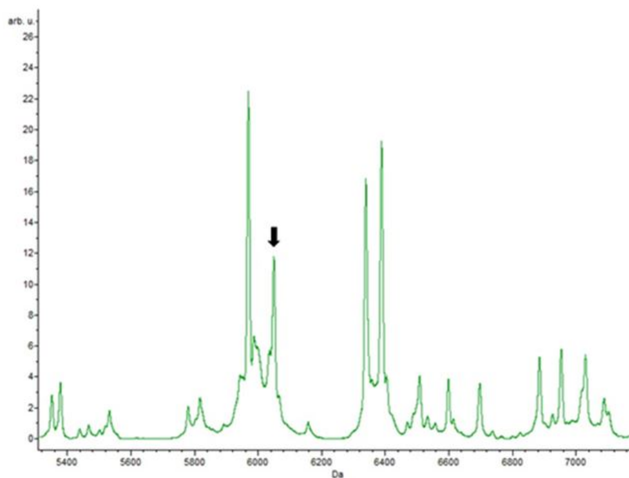
Figure 2. Enterococcus faecium spectrum showing the peak m/z\ 6048 \pm 1 ( p -value is 0.00001) characteristic of these strains.
