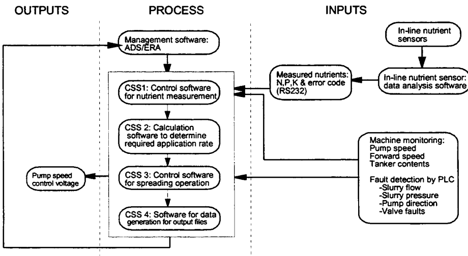
Figure 2 Control System Structure
