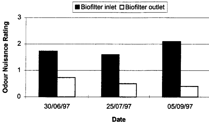
Figure 6 Odour intensity and concentration of gases at the biofilter's inlet and outlet
