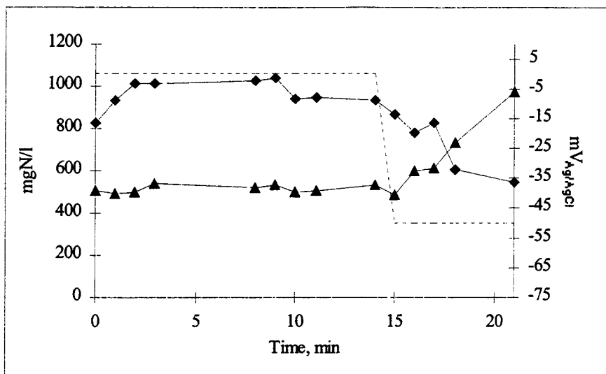
Figure 3 Influence of redox potential on nitrogen transformation during aerobic treatment of pig slurry, ◆ nitrate plus nitrite concentration, ▲ ammonium concentration and ----- redox potential.
