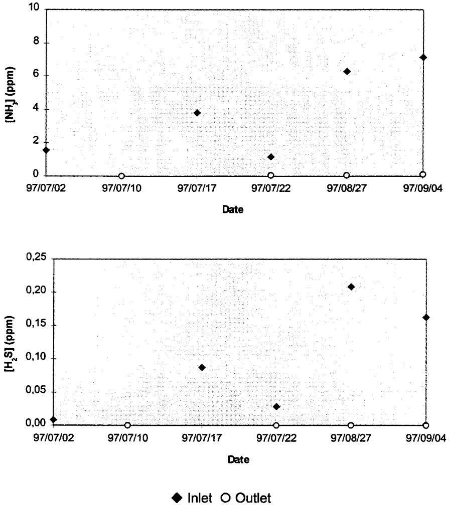
Figure 5 \text{NH}_3 and \text{H}_2\text{S} concentrations at the biofilter's inlet and outlet over time
