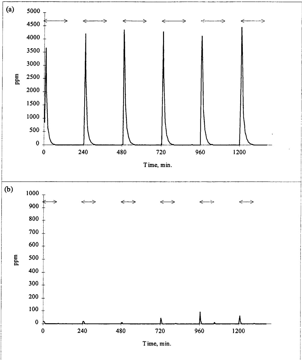
Figure 4 Continuous emissions of nitrous oxide during intermittent aeration, \longleftrightarrow aeration period. (a: run 3 and b: run 4).
