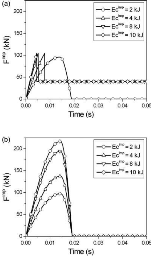
Fig. 14. Impact force, F^{\text{imp}} , using front-cell constitutive models associated with (a) FD and (b) RC conditions for different impact energies ( E_c^{\text{imp}} ).
