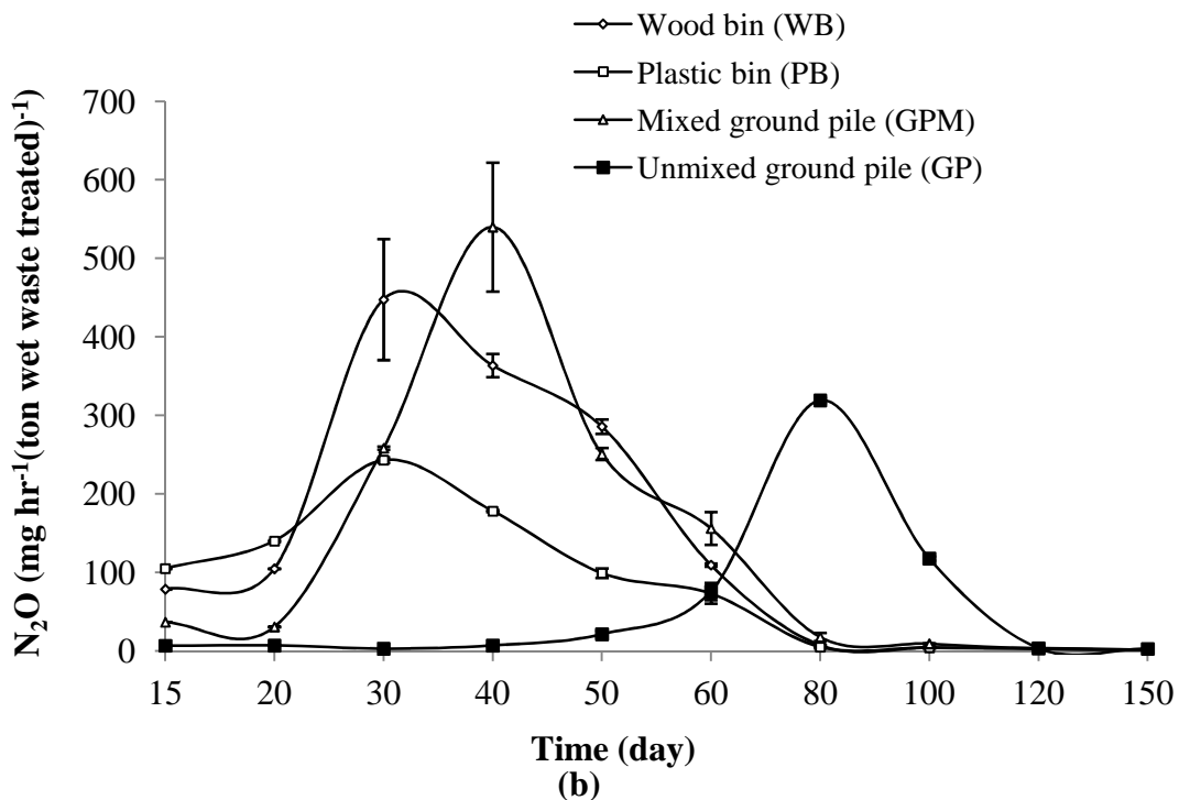
Figure 31 Measured emissions of \text{CO}_2 and \text{N}_2\text{O} from all four experimental home composting systems (HC) over 150 days: (a) carbon dioxide, \text{CO}_2 ; and (b) nitrous oxide, \text{N}_2\text{O} . Emissions of \text{CH}_4 between days 15 to 150 were below the detection threshold. Y-bars indicate the standard deviations (n=2).
