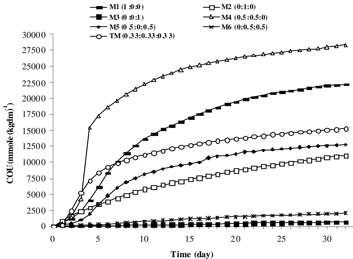
Figure 11 Cumulative oxygen uptake (COU) for formulas of food waste (FW), yard trimmings (YT) and wood chips (WC) during 32 days of respiratory. TM – average of triplicate testing for a 0.33:0.33:0.33 FW:YT:WC, namely TM1, TM2 and TM3.
