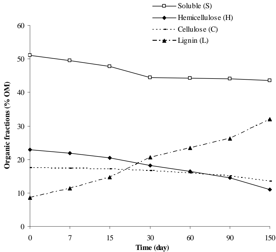
Figure 17 Evolution of the organic fractions for all treatments during 150 d of composting.
