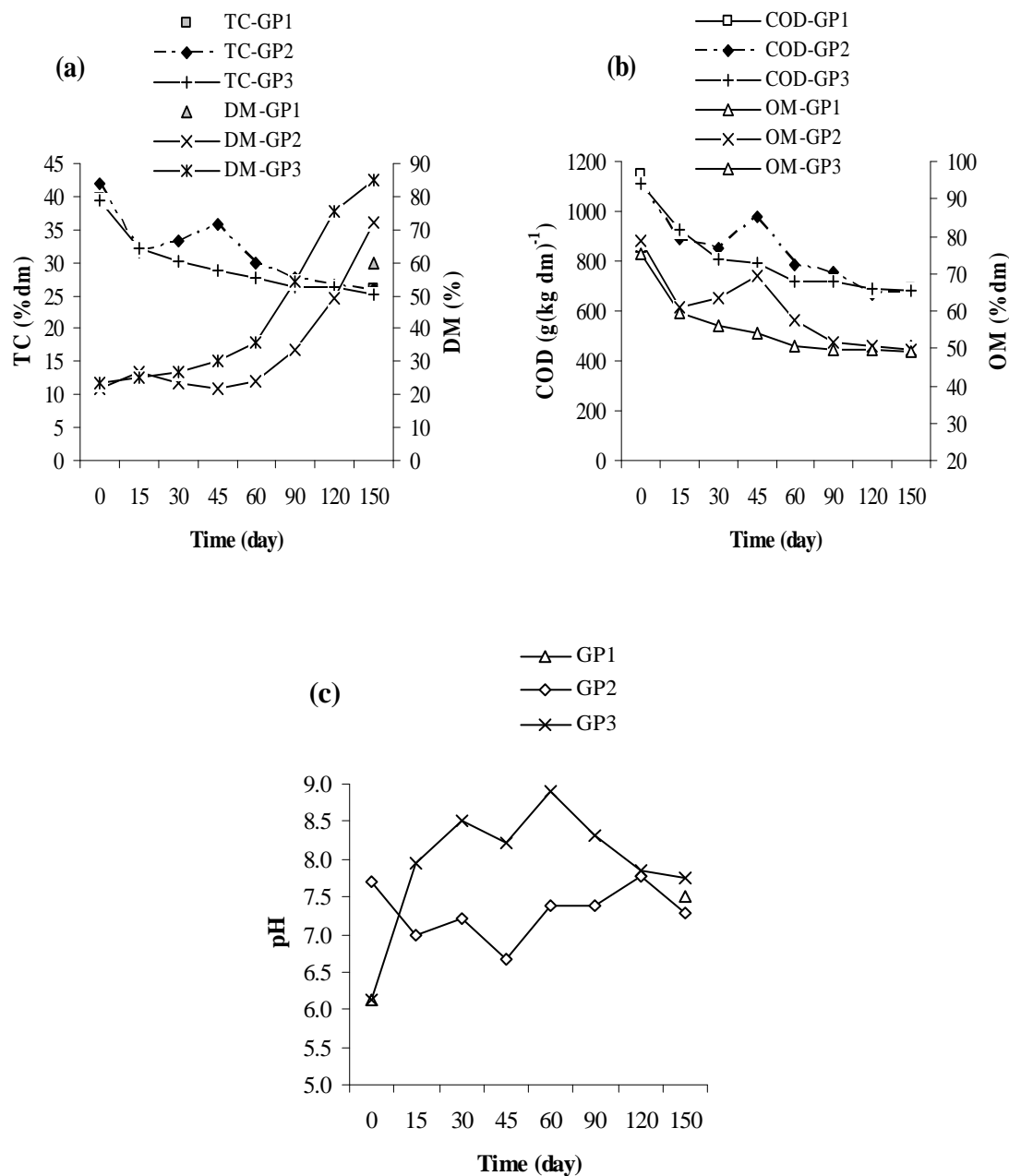
Figure 24 Evolution of the compost characteristics as influenced by management practices for the ground pile: (a) TC and DM; (b) COD and OM; and (c) pH. TC – total carbon; DM – dry matter; COD – chemical oxygen demand; OM – organic matter; GP1 – Ground Pile without BA, batch fed and not mixed; GP2 – Ground Pile without BA, weekly fed and mixed; GP3 – Ground Pile without BA, batch fed and mixed. Since GP2 was not mixed and sampled regularly, only day 0 and 150 values are illustrated.
