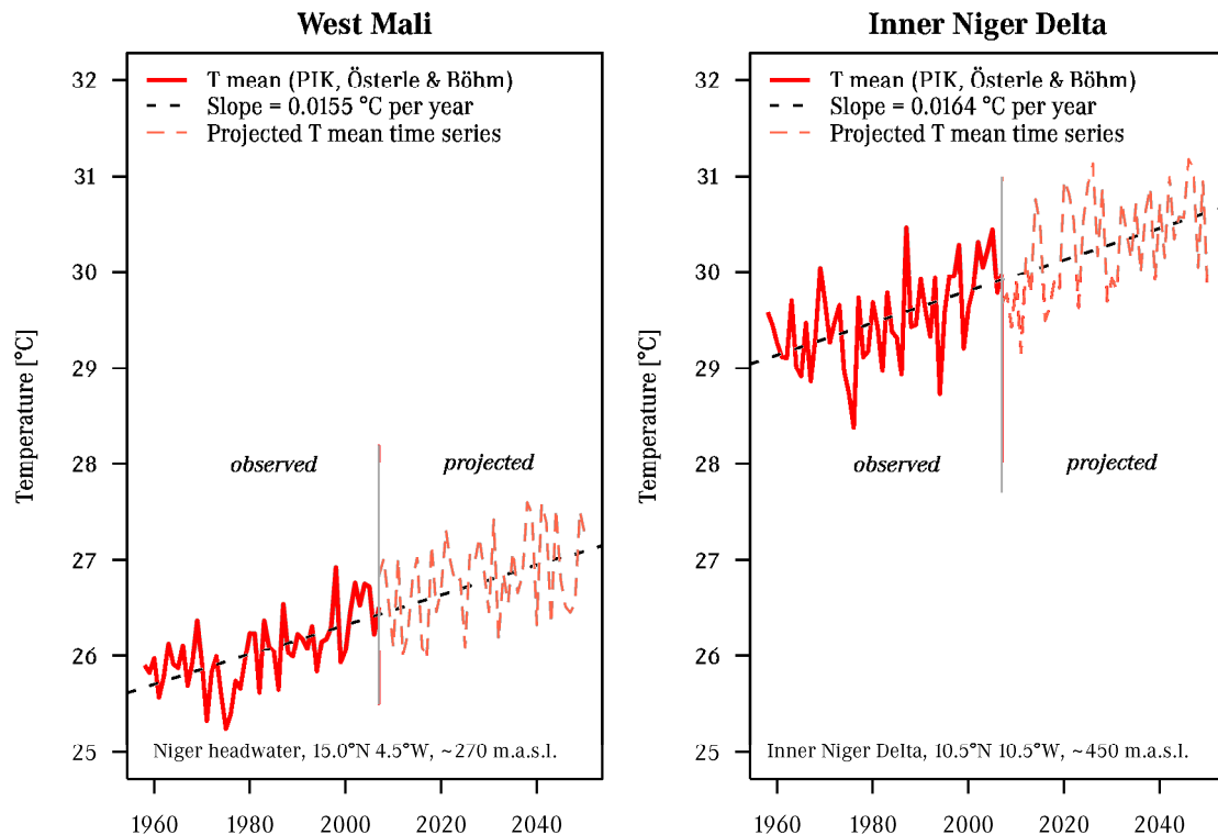
Figure 2.22. Temperature, Observations and Projections, Data Source: Österle & Böhm (2009)
