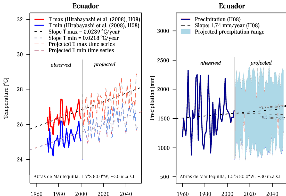
Figure 2.27. Temperature and Precipitation, Observations and Projections; Data Source: Hirabayashi et al. (2008)
