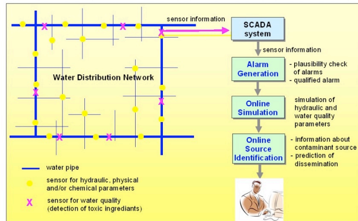
Figure 2: General system concept of SMaRT-Online W DN
