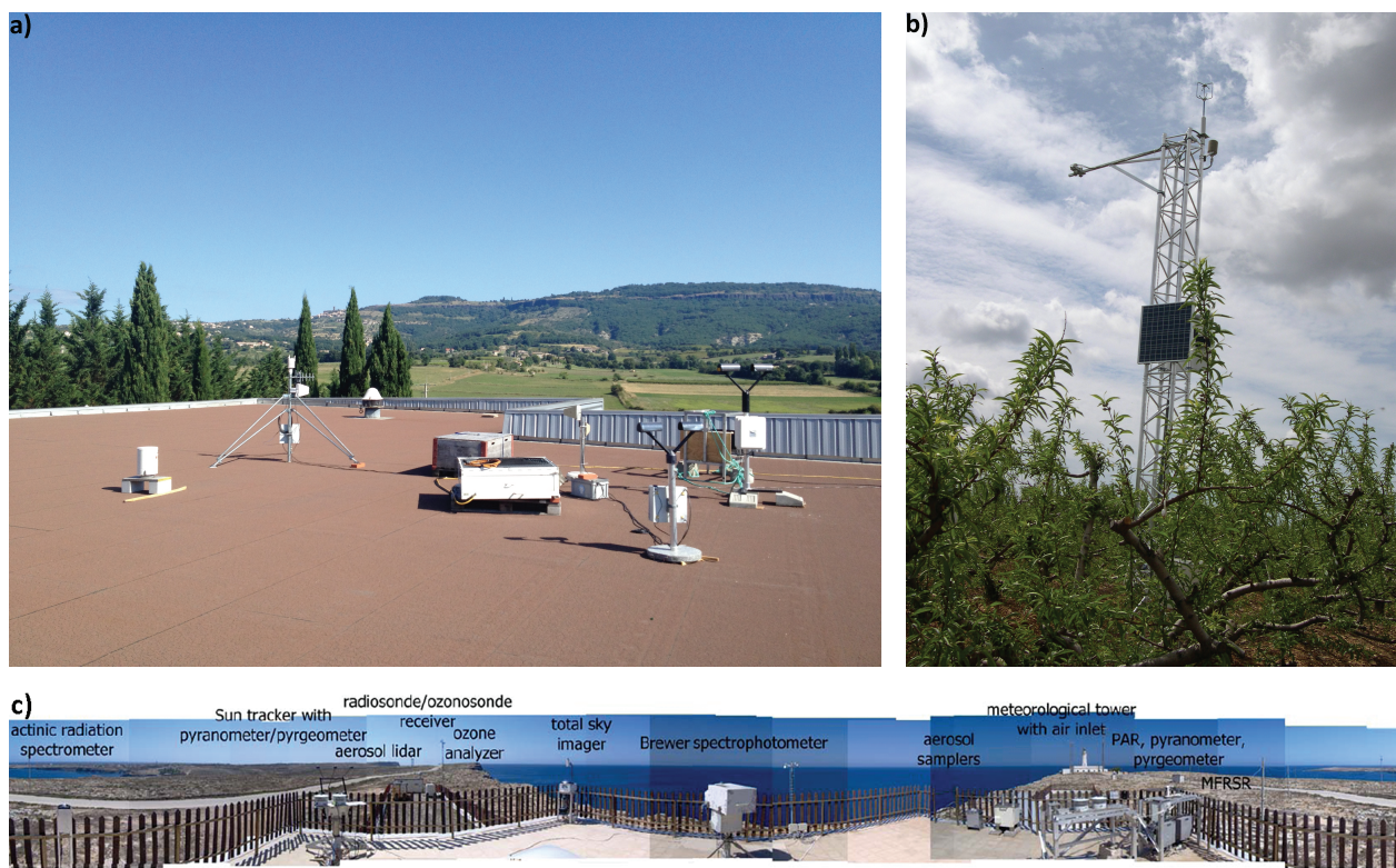
FIG. 4. Examples of HyMeX LOP and EOP sites: (a) CV, (b) flux tower deployed at the Crau–Camargue hydrological site, and (c) LA. [Source: (a) B. Boudevillain; (b) S. Garrigues; (c) A.G. Di Sarra.]
