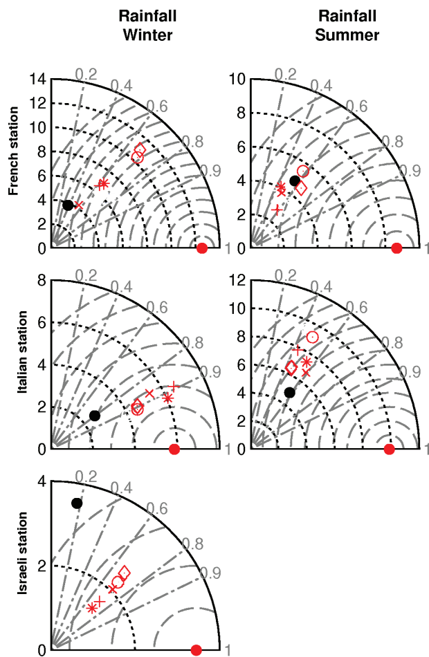
FIG. 8. Taylor diagrams for (left) winter and (right) summer rainfall showing standard deviation (dotted black lines), centered root-mean-square difference (dashed gray lines), and correlation (diagram angle) of ERA-Interim, ECA&D, and WRF outputs with respect to three station observations at (top) the Cévennes–Vivarais observatory in France, (middle) in northeastern Italy, (bottom) Israël for the period 2003–08 (GEWEX-labeled HyMeX stations; Drobinski et al. 2009, 2011; Flaounas et al. 2012, 2013). Black dot = ECA&D; red symbols = WRF and ERA-Interim, where red dot = station observations, × = ERA-Interim, star (*) and circle (o) = two configurations of WRF at 50-km resolution; cross (+) and diamond (◊) = two configurations of WRF at 20 km. (Source: E. Flaounas.)
