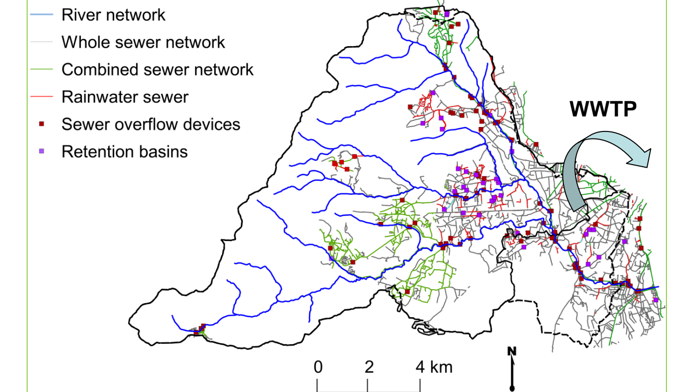
Figure 6: Current rainwater management map derived from local authorities data (Grand Lyon, SIAHYV).
