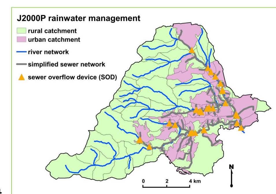
Figure 11: HRU delineation, sewer network and SODs.
