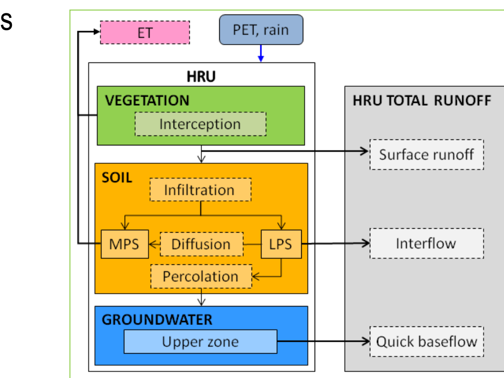
Figure 8: Physical processes and runoff contributions simulated at each time step and for each HRU.
