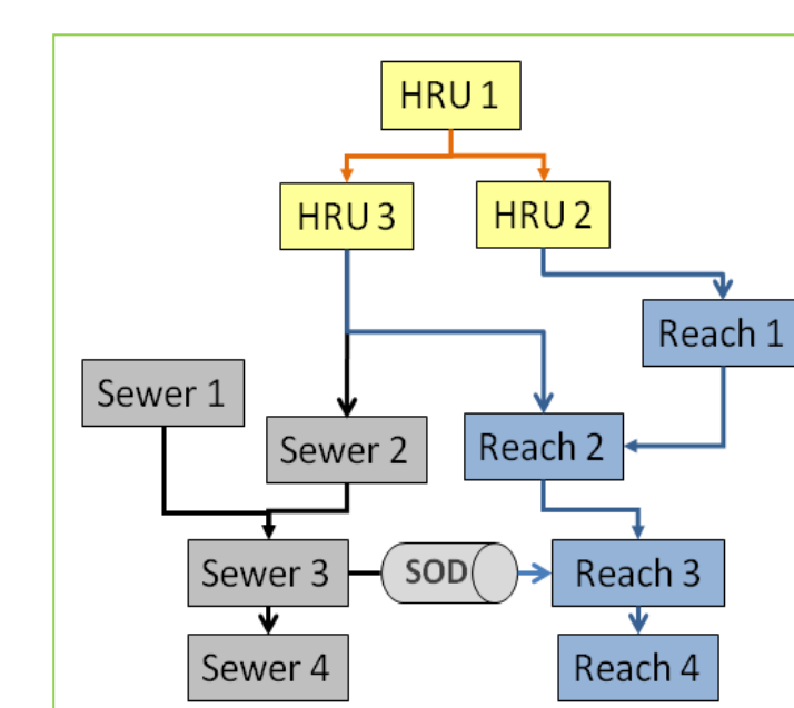
Figure 9: Routing in J2000P. Addition of a sewer network. Some SODs can connect sewer reaches to river reaches.
