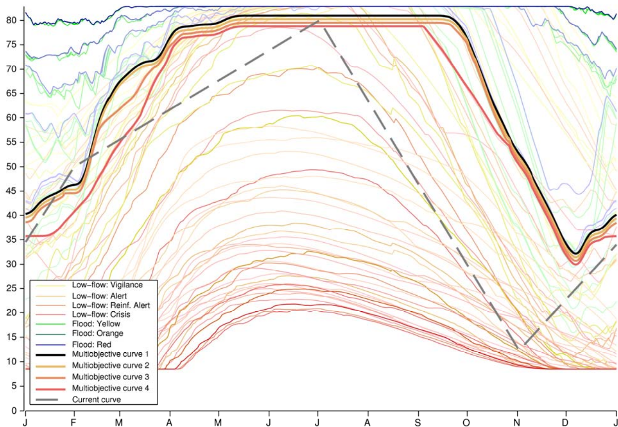
Figure 59: Result of multi-objective optimisation of the filling curve for Pannecière Lake calculated from future (FUT) simulated flows (7 GCMs scenarios x 2046-2065). Volumes (hm 3 ). Multi-objective filling curves in bold, current filling curve in dotted grey, low-flow and high-flow constraints in thin line.
