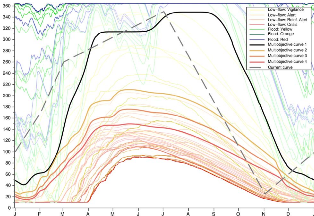
Figure 57: Result of multi-objective optimisation of the filling curve for Marne Lake calculated from future (FUT) simulated flows (7 GCMs scenarios x 2046-2065). Volumes ( \text{hm}^3 ). Multi-objective filling curves in bold, current filling curve in dotted grey, low-flow and high-flow constraints in thin line.
