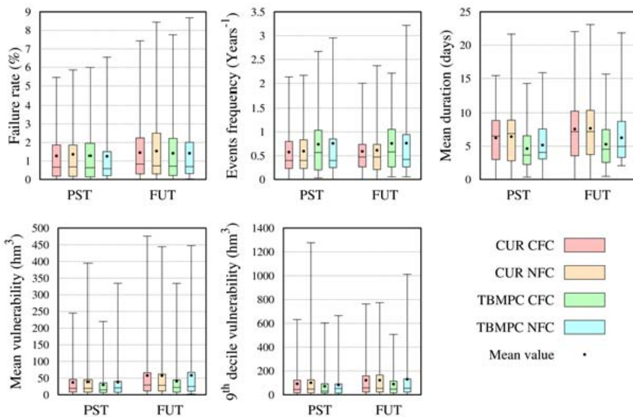
Figure 60: Performance indicators (Failure rate, events frequency, mean duration, mean vulnerability and 9 th decile vulnerability) for the 1 st high-flow threshold (Yellow) calculated from 7 GCMs scenarios in present (PST) and future (FUT) time for 4 management adaptations.
