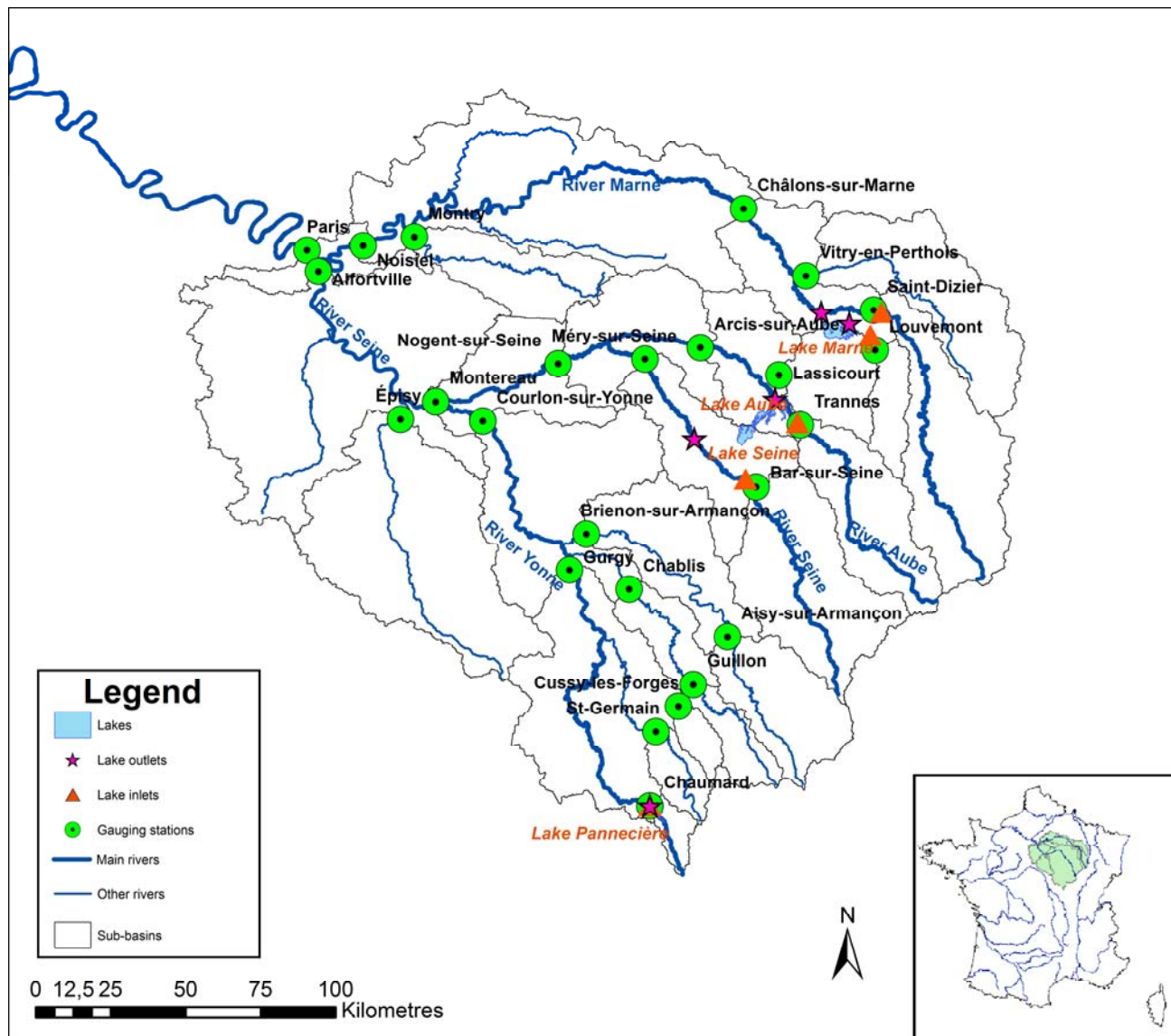
Figure 43: Contour map of the River Seine basin at Paris, with gauging stations, main hydrographic network and reservoirs
