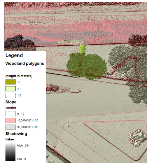
Figure 15: Delineated Vegetation Polygon
