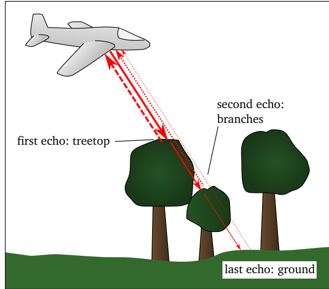
Figure 1: Principle of range measurement by airborne laser scanning.
