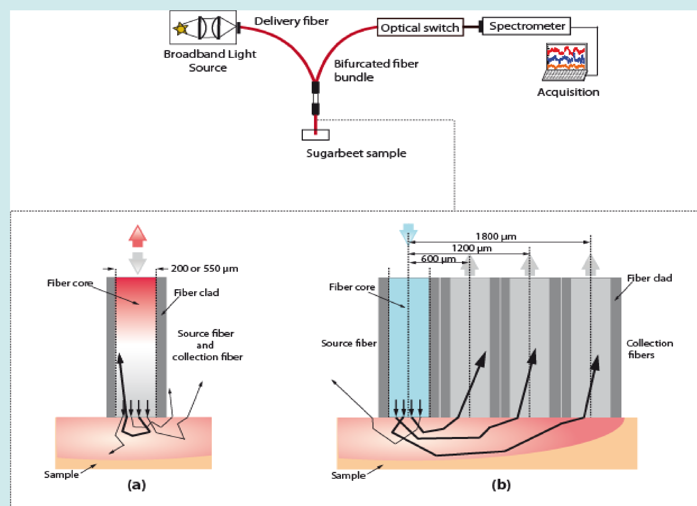
Figure: a) Schematic diagram of the single- fiber probe. b) schematic diagram of the multiple-fiber probes (F1 at 600 μm, F2 at 1200 μm and F3 at 1800 μm).
