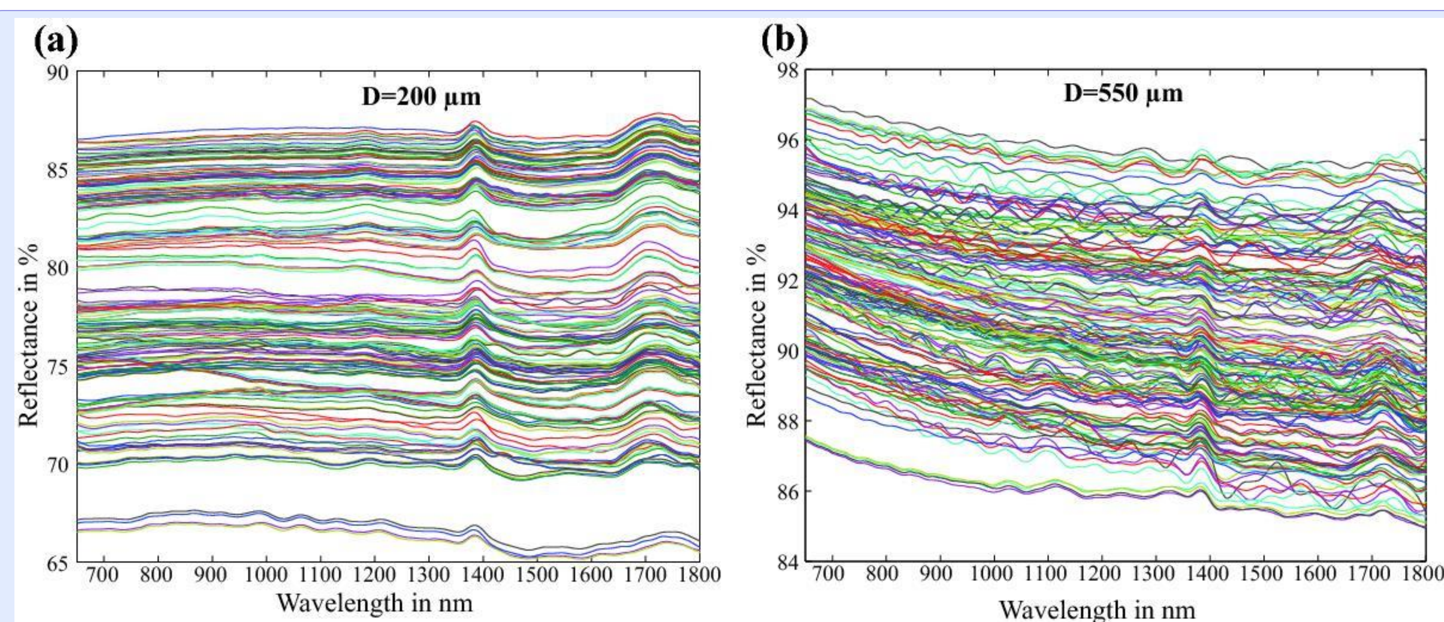
Figure : Raw reflectance spectra of the single-fiber probe with two diameter (a) 200 μm. (b) 550 μm .
