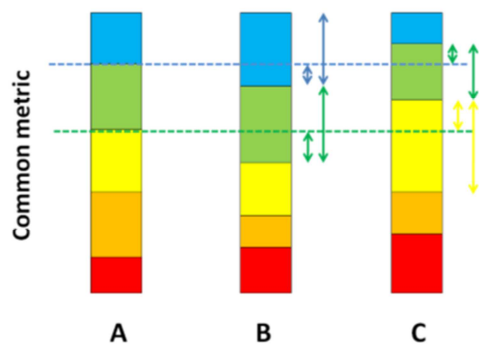
Figure C.4: National classification schemes (A, B, C) intersected by the average boundary positions derived in intercalibration ("harmonisation line" - broken blue and green lines). Small arrows depict the distance of relevant national boundary to the harmonisation guideline. Large arrows define relevant national class width. The relation of small to large arrow-lengths specifies the boundary bias in class equivalents (figure and description copied from BIRK et al. (2011)).
