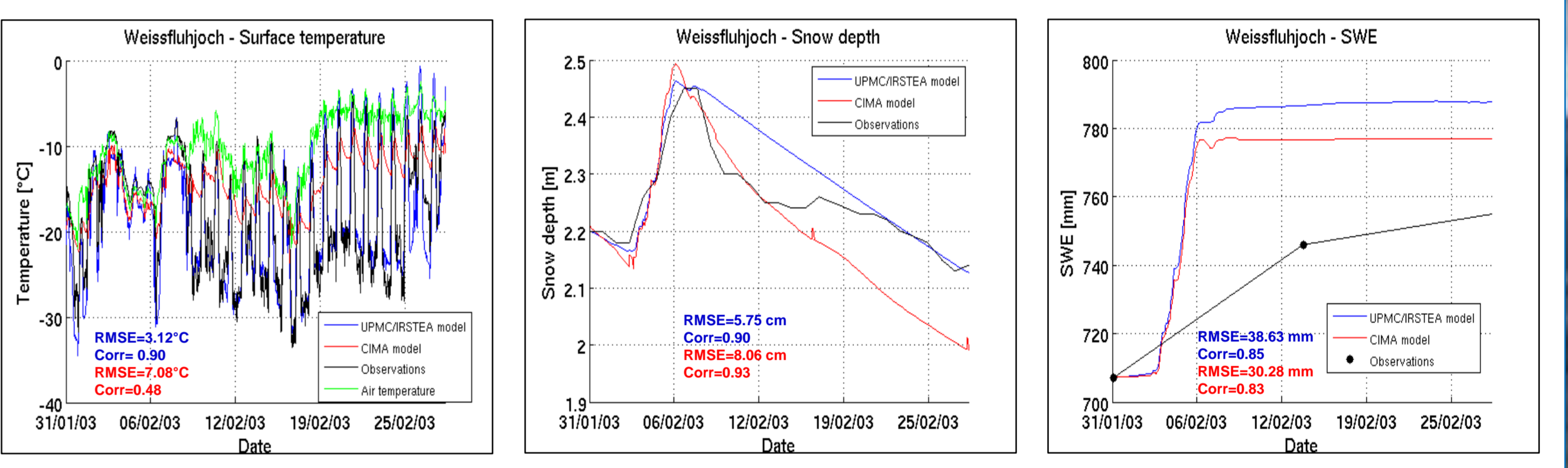
Snow models intercomparison at Weissfluhjoch site, 31 January 2003 - 28 February 2003.
