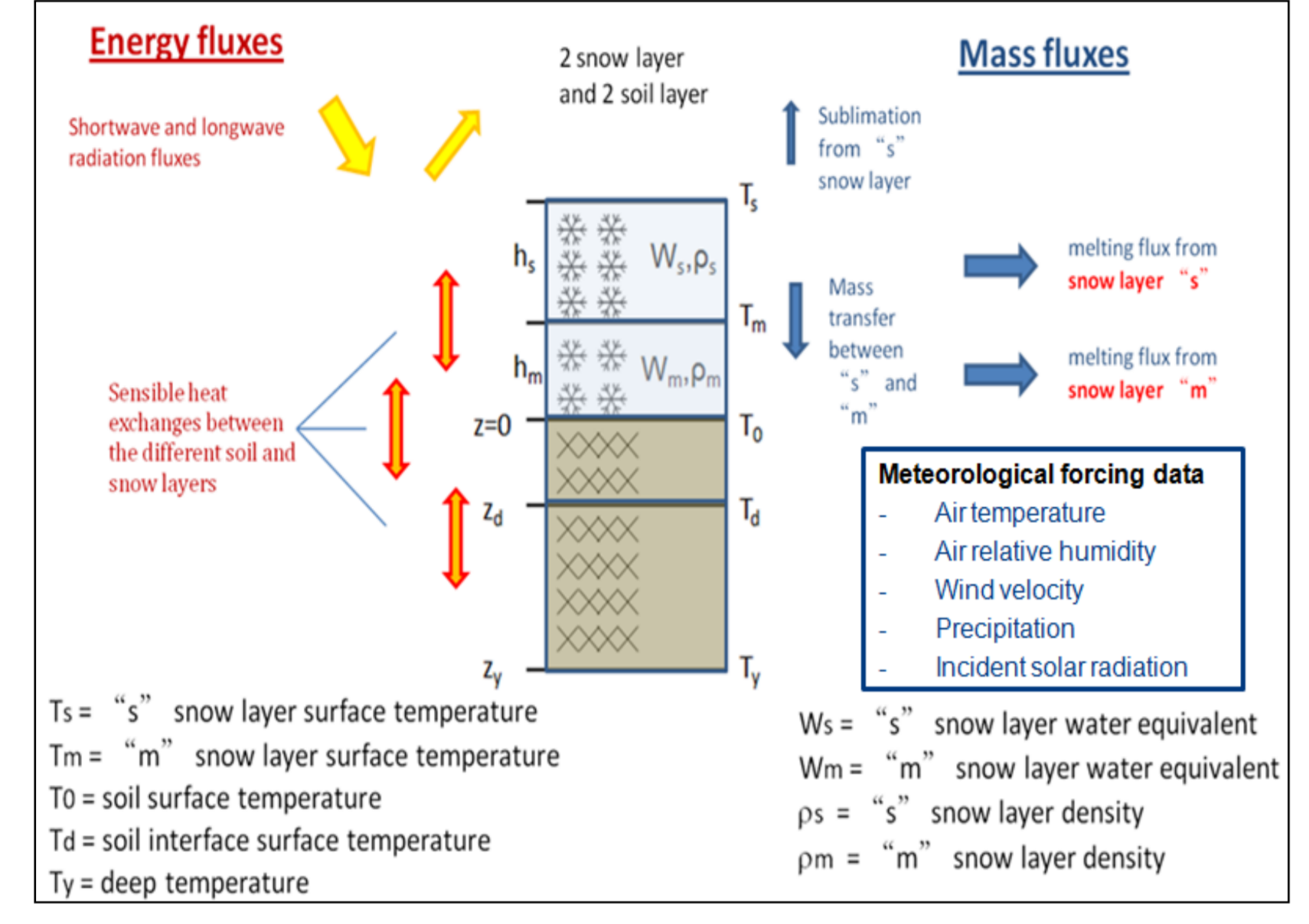
Snow model scheme - Energy and mass fluxes between adjoining layers and atmosphere are shown.
