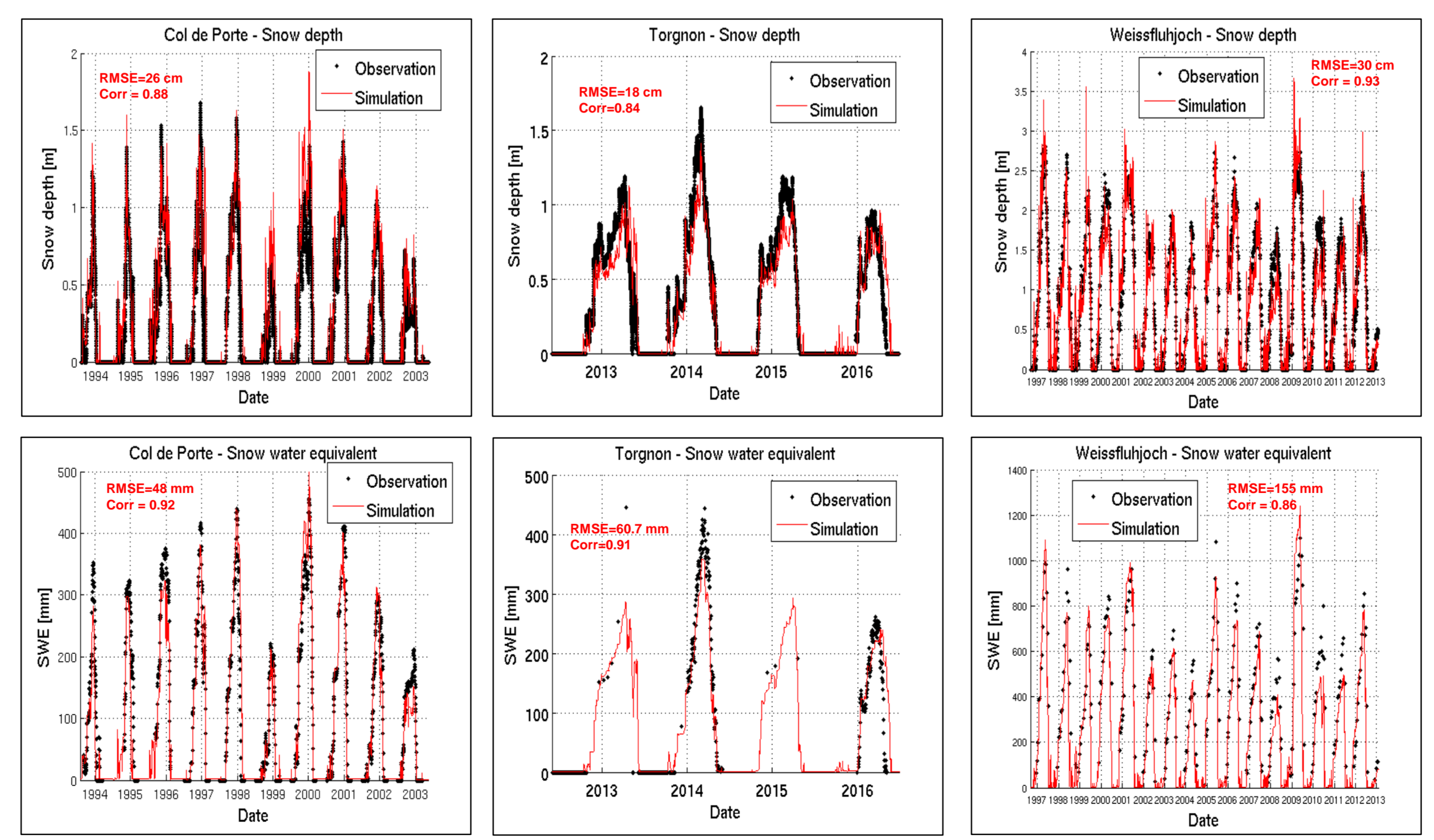
Calibration results - simulations of snow depth and SWE at the Alpine sites.
