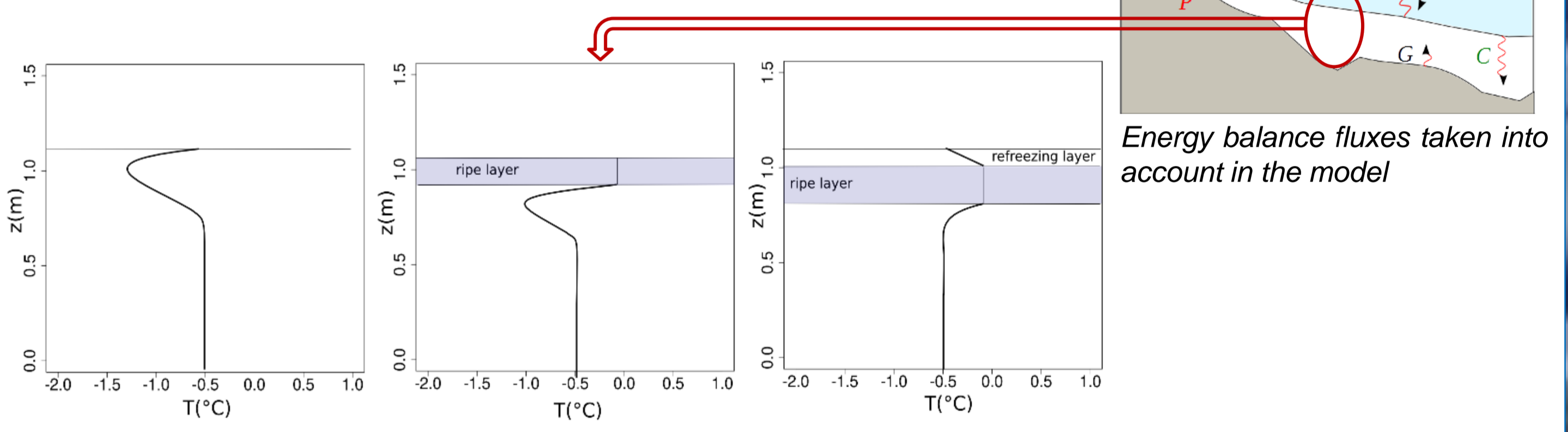
The three configurations of the snowpack conduction: from left to right, pure conduction in dry snow, ripening of a surface layer (conducting to melt), and refreezing layer.
