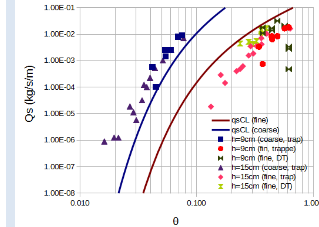
Bedload flux estimated as a function of the Shields parameter. Comparison between experimental data and semi-empirical formulas (Meyer-Peter & Müller, 1948 ; Camenen & Larson, 2005)
