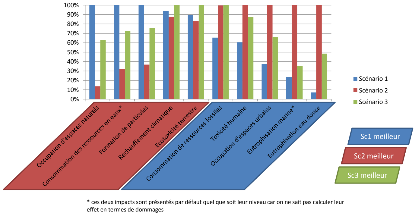
Figure D. 6 H4V Ranked and highlighted midpoint subset histogram (severity)
