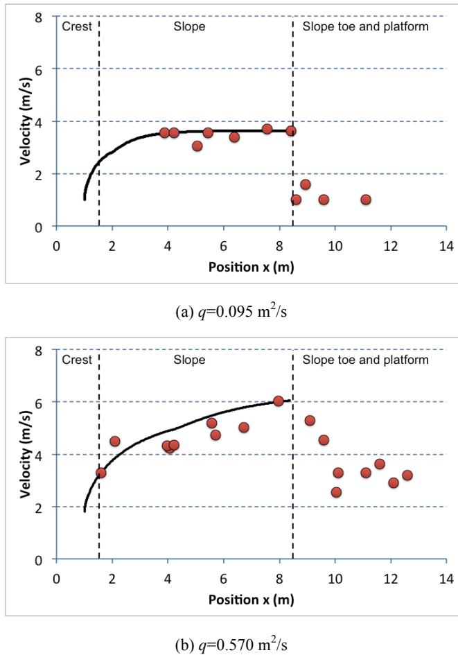
Figure 5. Flow velocity for a flow rate of 0.095 m 2 /s (minimum flow rate, test No. 1) (a) and a flow rate of 0.570 m 2 /s (maximum flow rate) (b). Symbols represent the measurements. Solid lines represent the Chanson model.
