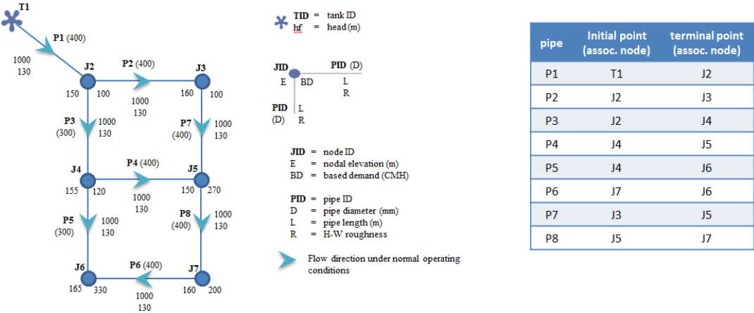
Figure 8: Case study – Proposal 2. (a) Network layout; and (b) Burst position – List of flow direction. Source: (Ayala-Cabrera et al., 2017a)
