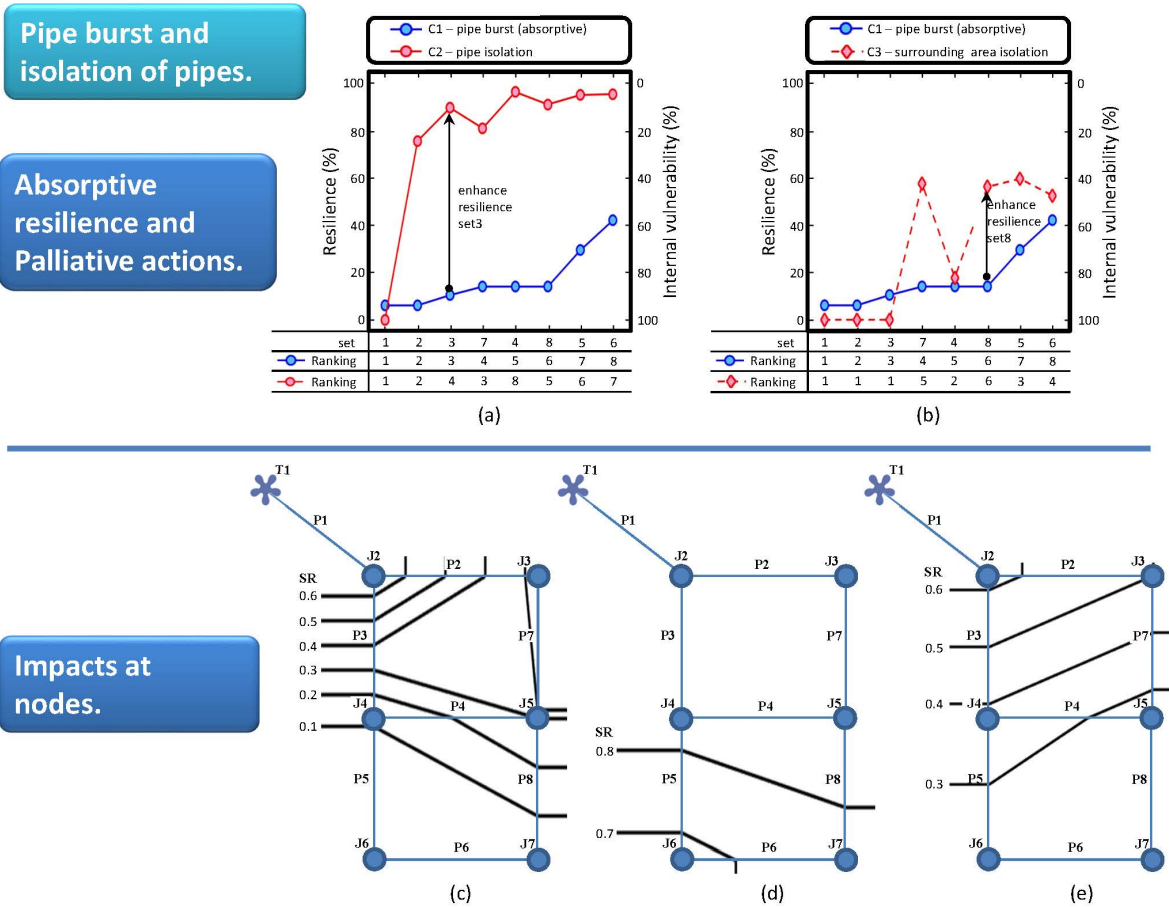
Figure 10: Pipe burst and isolation of the affected pipe – Proposal 2.
