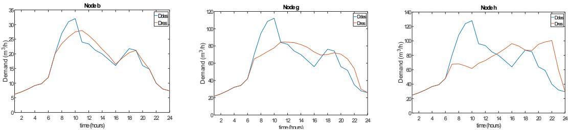
Figure 12: Desired demand vs. resulting demand for Node b, g and h.
