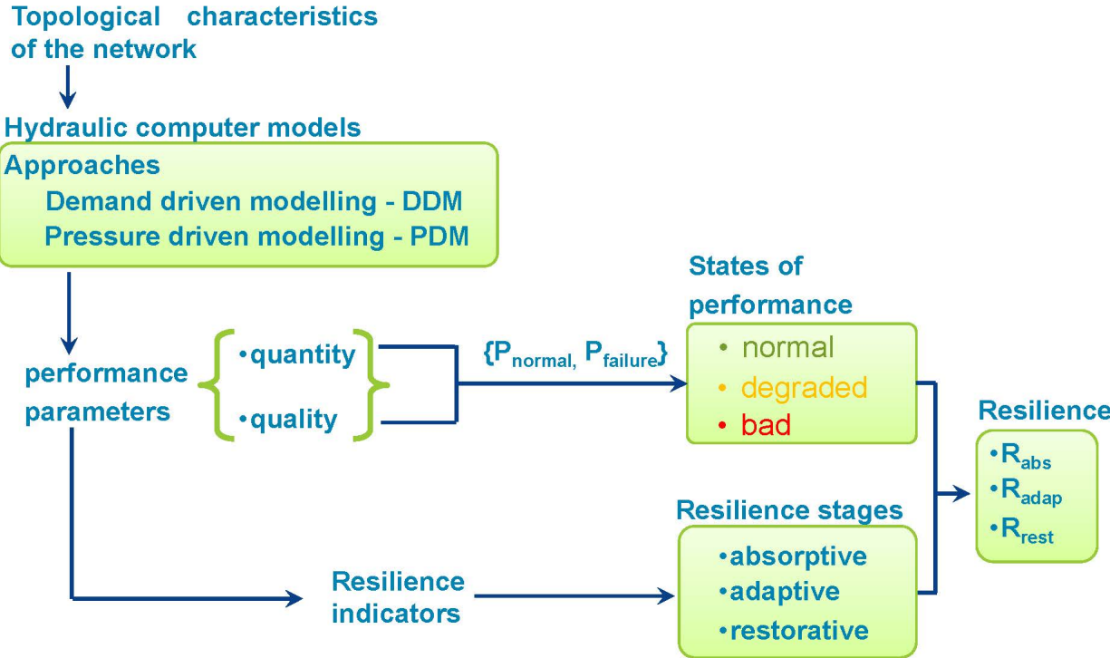
Figure 4: Theoretical framework to assess resilience – Quantity; proposal 1. Source: (Ayala-Cabrera et al., 2017b)
