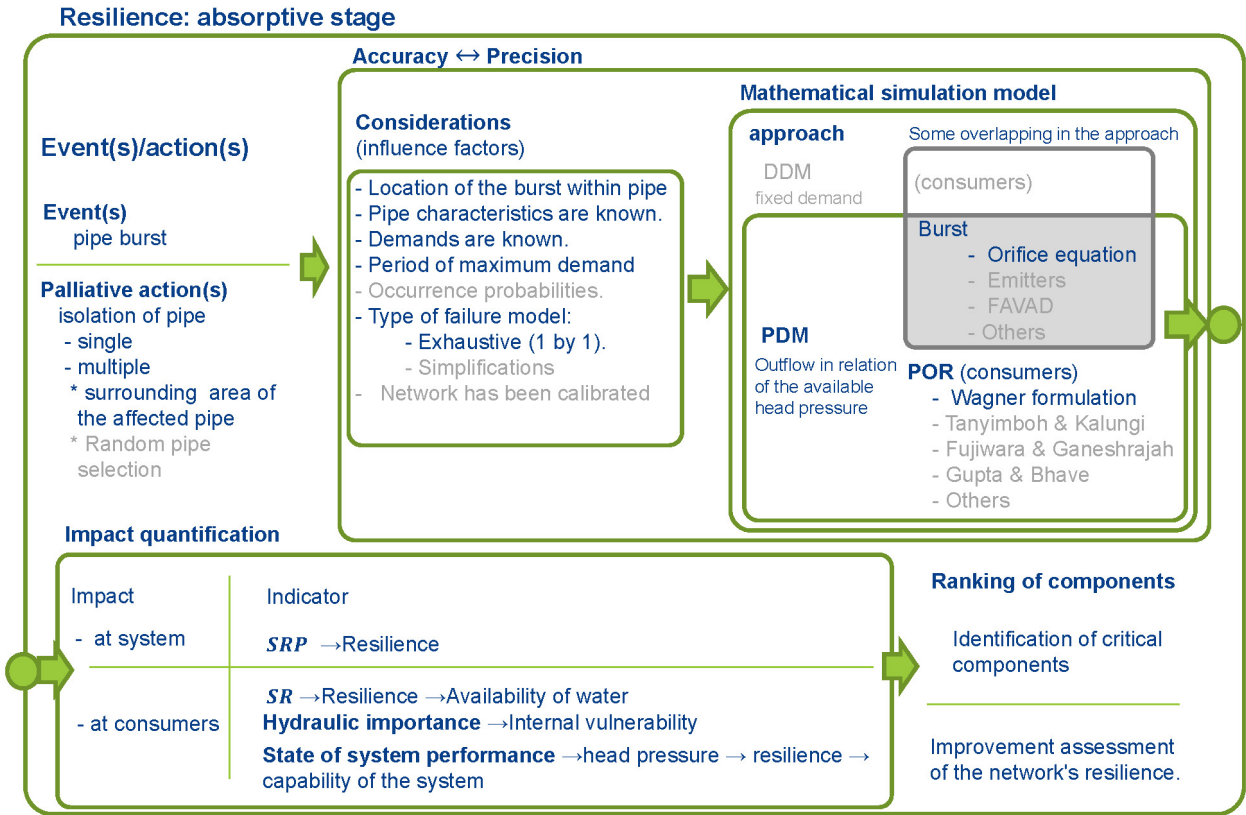
Figure 7: Theoretical framework to assess criticality – Quantity; proposal 2. Source: (Ayala-Cabrera et al., 2017a)
