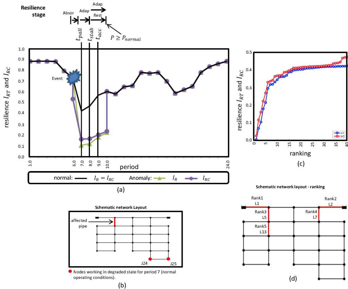
Figure 6: Analysis through resilience indicators. – Proposal 1. (a) Resilience stages; (b) network layout – stages; (c) ranking of pipe – peak demand period; and (d) network layout – ranking. Source: (Ayala-Cabrera et al., 2017b)
