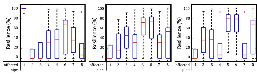
Figure 9: Pipe burst; Results – Proposal 2. Source: (Ayala-Cabrera et al., 2017a)
