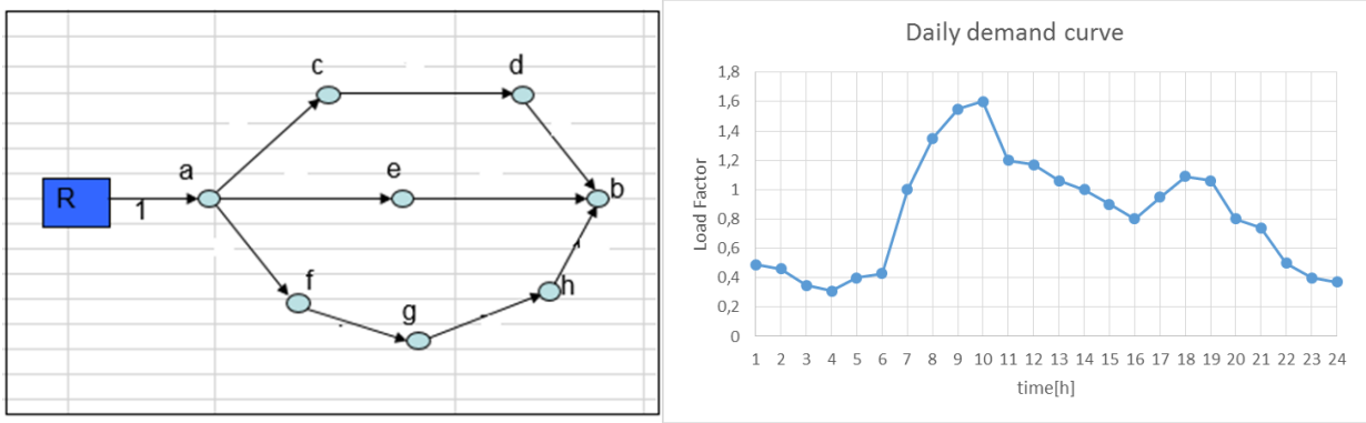
Figure 11: Test network (left) and daily demand curve (right).
