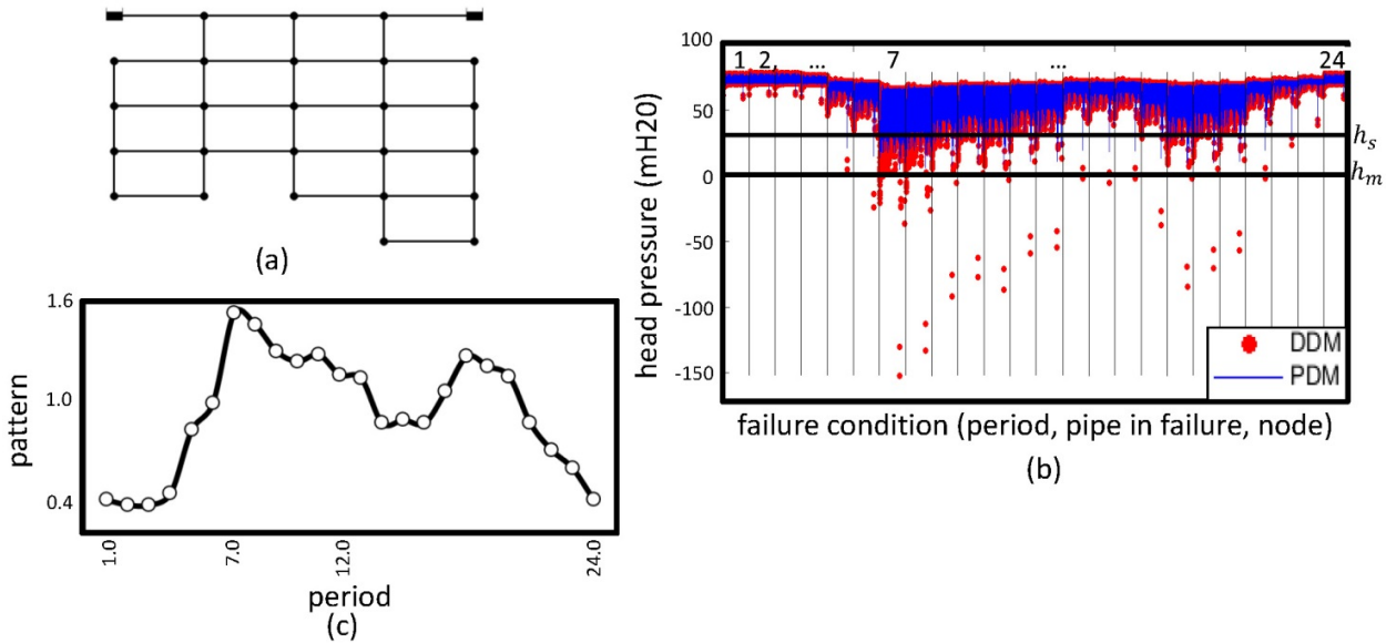
Figure 5: Pipe characteristics and head pressure results. – Proposal 1. (a) Network layout; (b) single pipe failure condition for all periods; and (c) demand pattern. Source: (Ayala-Cabrera et al., 2017b)
