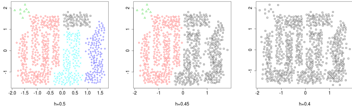
Figure 6. C1: Resulting partitions for three different thresholds on the homogeneity merging degree, h . The axes are the x and y coordinates.
