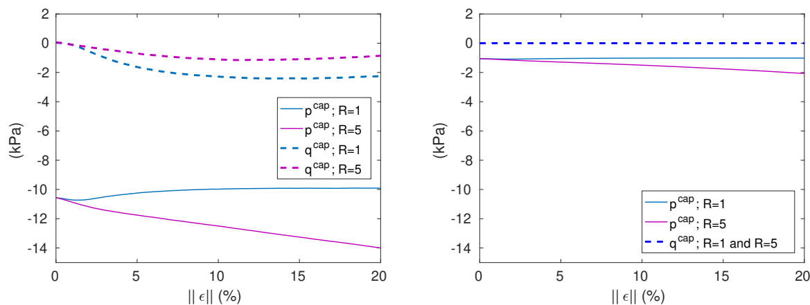
Figure 6: Capillary stresses during the two loading paths R = 1 and R = 5 imposed on the dense packing, as per \mu UNSAT expressions (left), compared with Bishop’s estimation (right)
