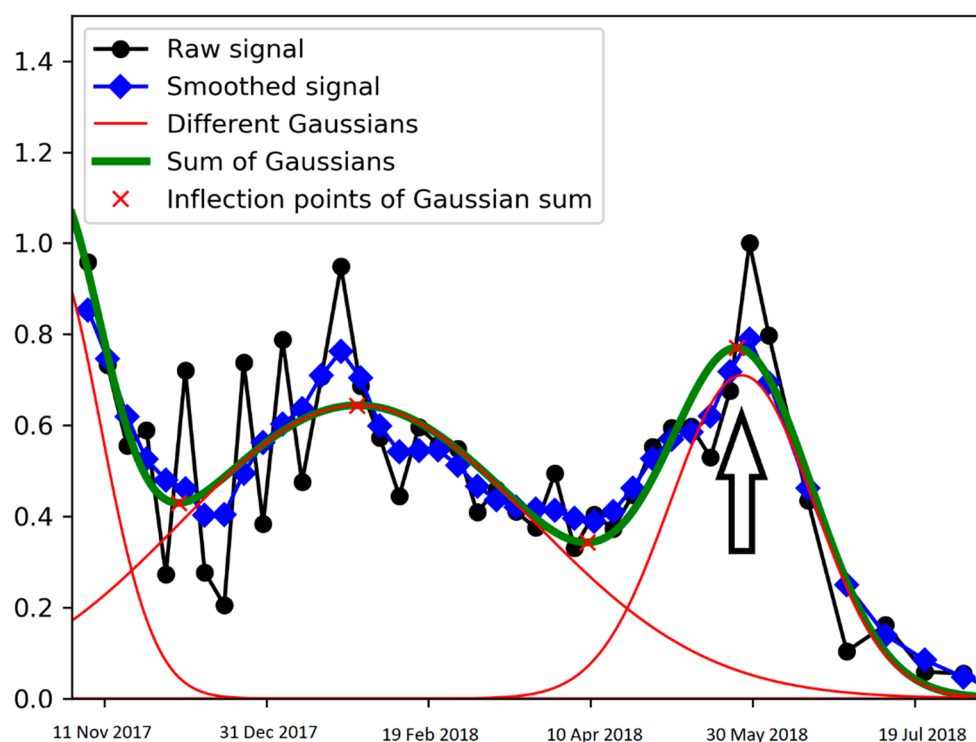
Figure 8. Gaussian fitting of the S1-VH temporal series of a winter wheat plot at the West Bekaa plain of Lebanon. The incidence angle is 43\text{--}45^\circ . The x-axis represents the date and the y-axis refers to the normalized signal. The black arrow indicates the inflection point where soft dough had taken place.
