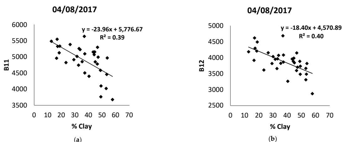
Figure 5. Soil clay content as a function of the SWIR bands of S-2, analyzed on 4 August 2017: (a) Band 11 (B11); (b) Band 12 (B12).
