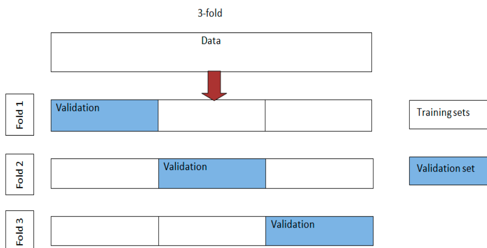
Figure 3. Three-fold cross-validation.
