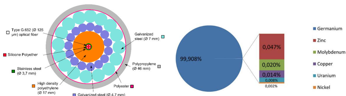
Figure 1. Example of materials used in an underwater optical telecommunication cable and environmental contribution of resources to Abiotic Resources Depletion (ARD) impact category for the cable manufacturing (from Orange Group)
