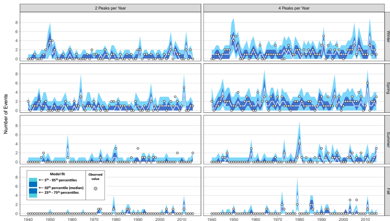
Figure 4. An example of a figure in a paper produced in R with the package ggplot2 using the facet_grid function, which allows the user to split a dataset by categories (rows and columns). Here, a probabilistic time-series GAMLSS model of flood frequency at one gauging station in Ohio, USA, is shown for four different seasons (rows) and two peak-over-threshold quantities (columns: two to four peaks per year). The probabilistic model is plotted in the background as colour ribbons (using geom_ribbon ), and the observed values are plotted in the foreground as grey circles ( geom_point ). Source: Neri et al. (2019).
