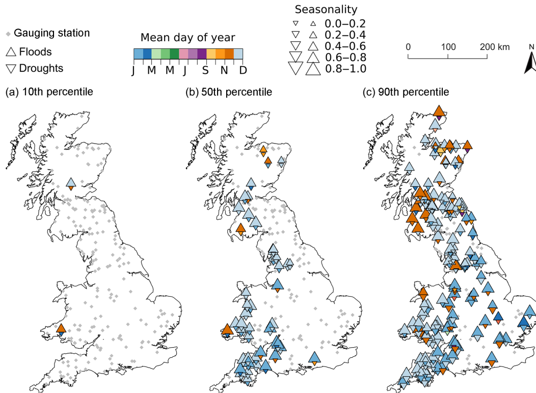
Figure 9. Time of year (mean day of year in colour scale and seasonality in size scale) of the hydro-hazards for the hot-spots in Great Britain on the baseline for the (a) 10th, (b) 50th, and (c) 90th percentiles.
