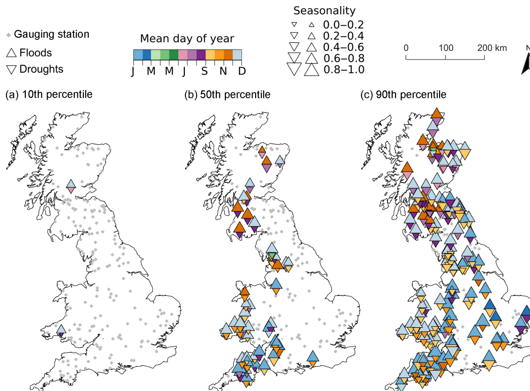
Figure 8. Time of year (mean day of year in colour scale and seasonality in size scale) of the hydro-hazards for the hot-spots in Great Britain in the 2080s for the (a) 10th, (b) 50th, and (c) 90th percentiles.
