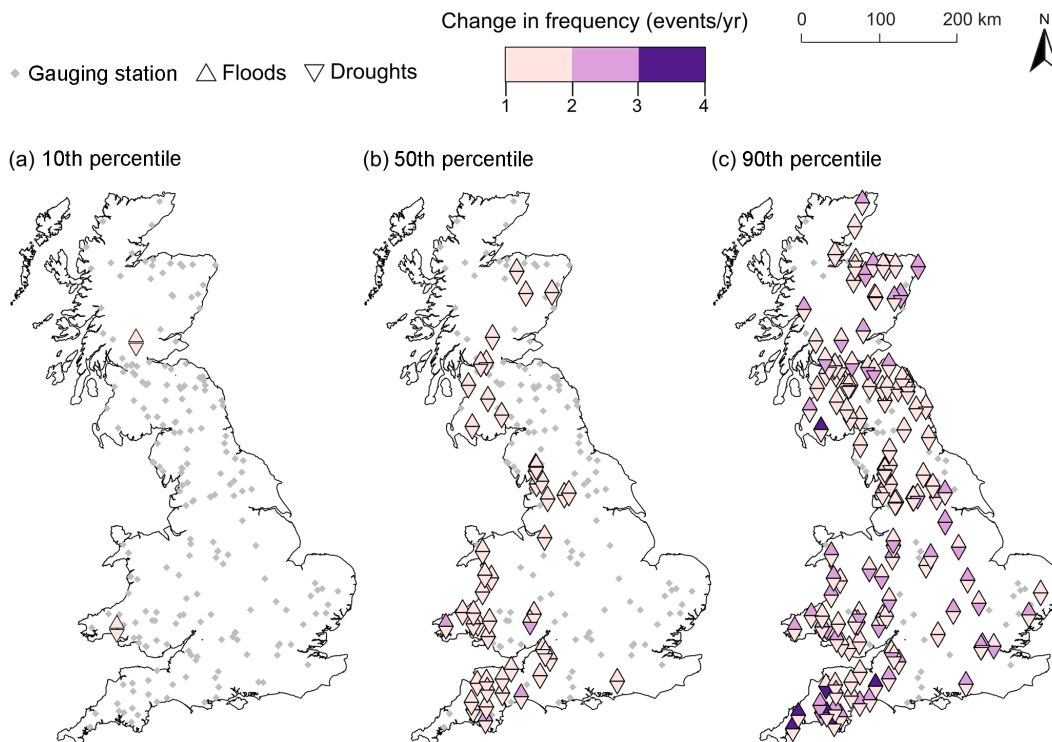
Figure 5. Changes in frequency of the hydro-hazards for the hot-spots in Great Britain for the (a) 10th, (b) 50th, and (c) 90th percentiles.
