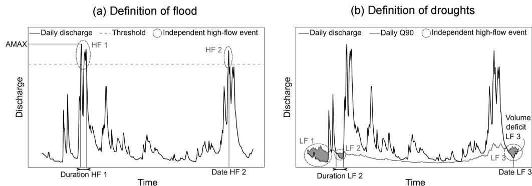
Figure 1. Selection and characterization in terms of frequency, magnitude, duration, and time of year of (a) floods (HF: high-flow event, AMAX: annual maximum POT) and (b) droughts (LF: low-flow event).
