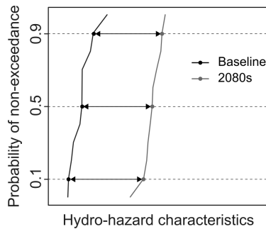
Figure 2. Quantification of signal of change in a hydro-hazard characteristic, as the difference between the baseline and 2080s cumulative distribution functions for the 10th, 50th, and 90th percentiles (dotted lines).
