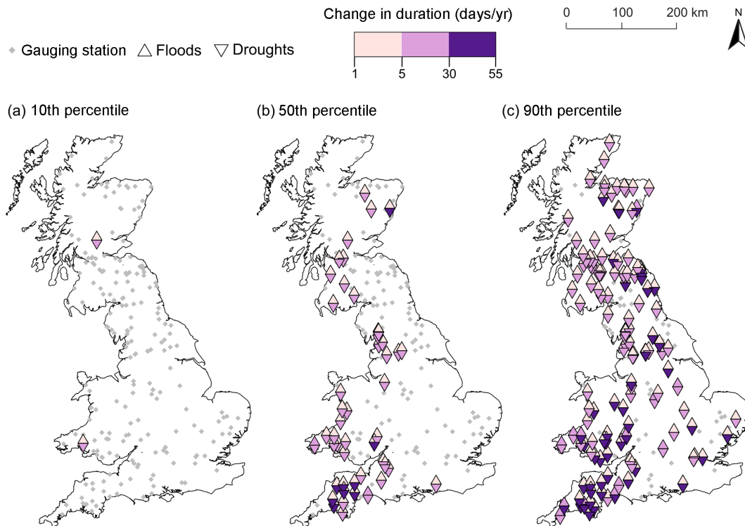
Figure 7. Changes in duration of the hydro-hazards for the hot-spots in Great Britain for the (a) 10th, (b) 50th, and (c) 90th percentiles.
