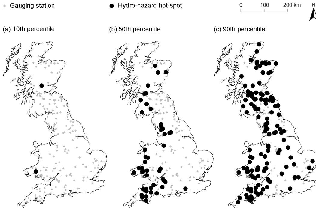
Figure 4. Hydro-hazard hot-spots in Great Britain for the (a) 10th, (b) 50th, and (c) 90th percentiles.
