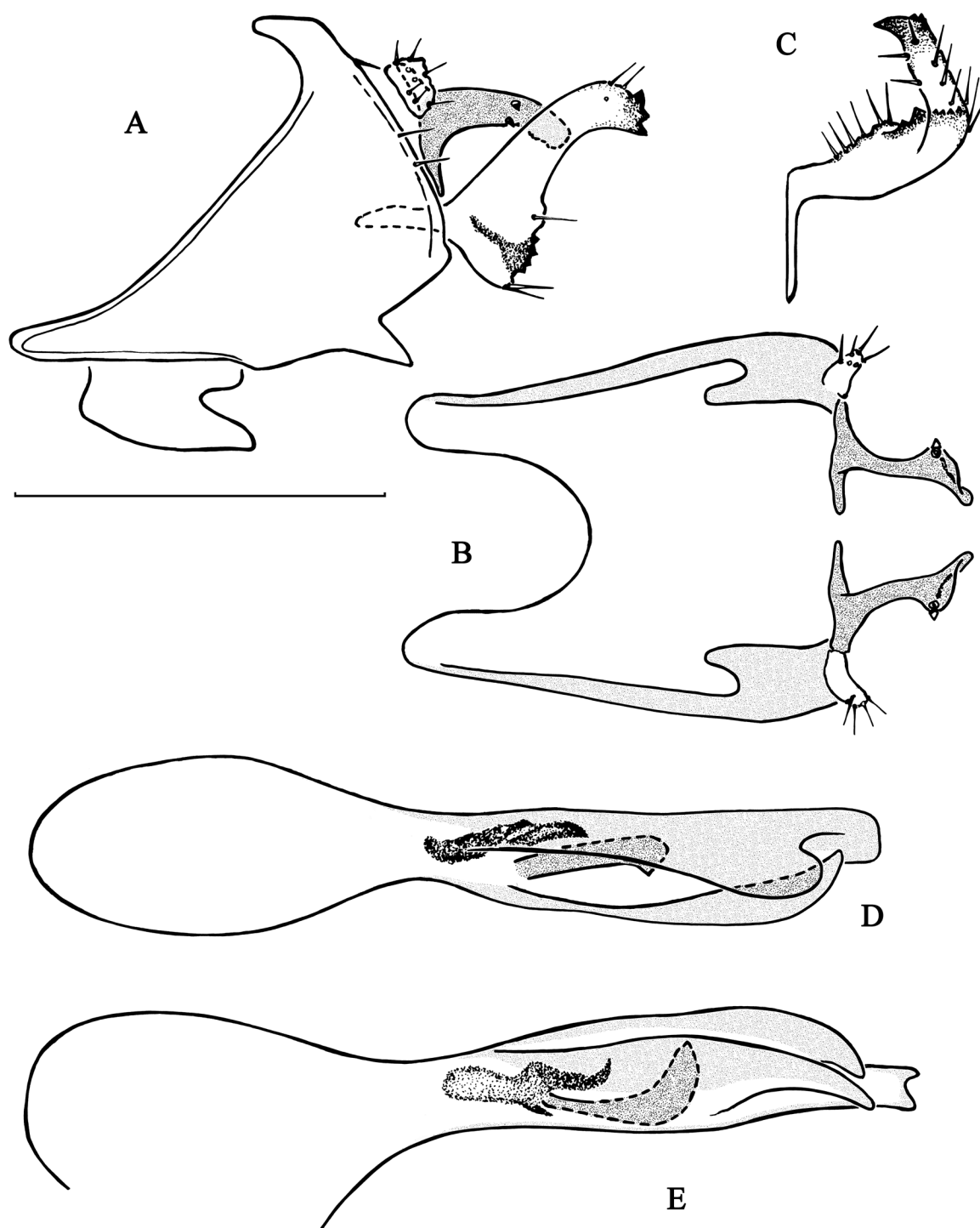
Fig. 9. Chimarra jejyorum sp. nov. A–B. Abdominal segments IX and X. A. Lateral view with ventral margin of sternite VIII. B. Dorsal view. C. Inferior appendage, dorsal view. D–E. Phallic apparatus. D. Dorsal view. E. Lateral view. Scale bar = 0.5 mm.
