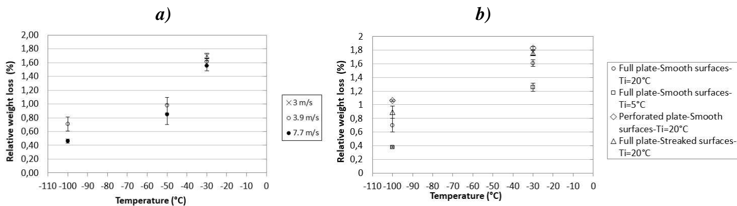
Figure 5: Average total relative weight loss according to gas temperature
