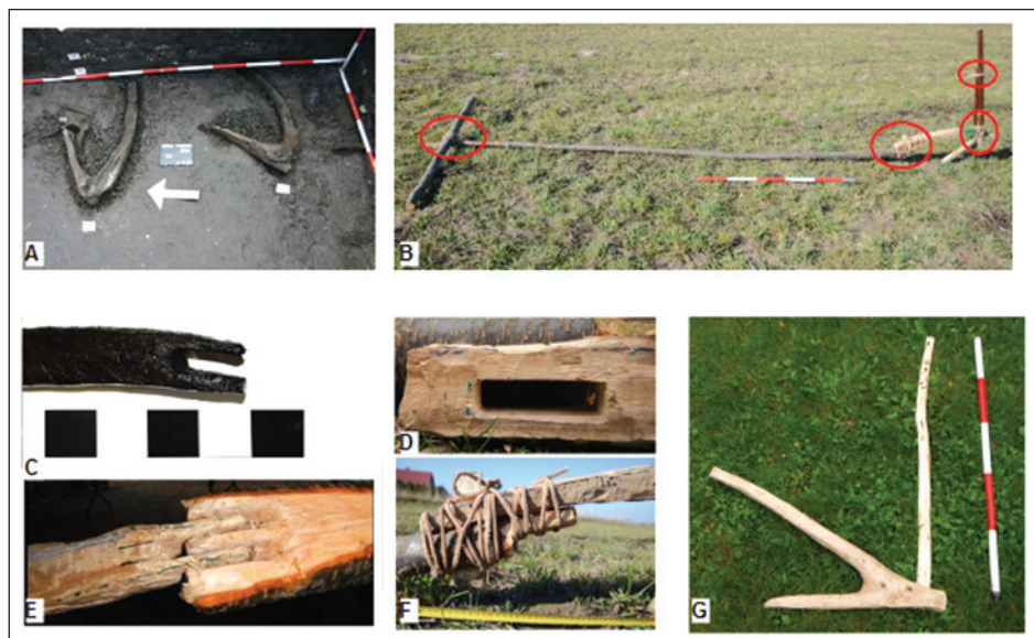
Figure 2. Ards. A: Recovered ards from archaeological digs (1131-1026 BC). B: Reconstructed ard B prepared for ploughing; red circles show joints between parts with leather lines. C: Beam of a recovered ard ending with oval cut. D: Reconstructed hole for a tie hook in ard B. E: Reconstructed ard A. F: The join between ard and beam using leather lines (ard B). G: The standardized (ard C) type with sole and tie hook (Tegtmeier, 1993). Photos: A, Peter Kováčik; B-G, Jan Pavelka.
