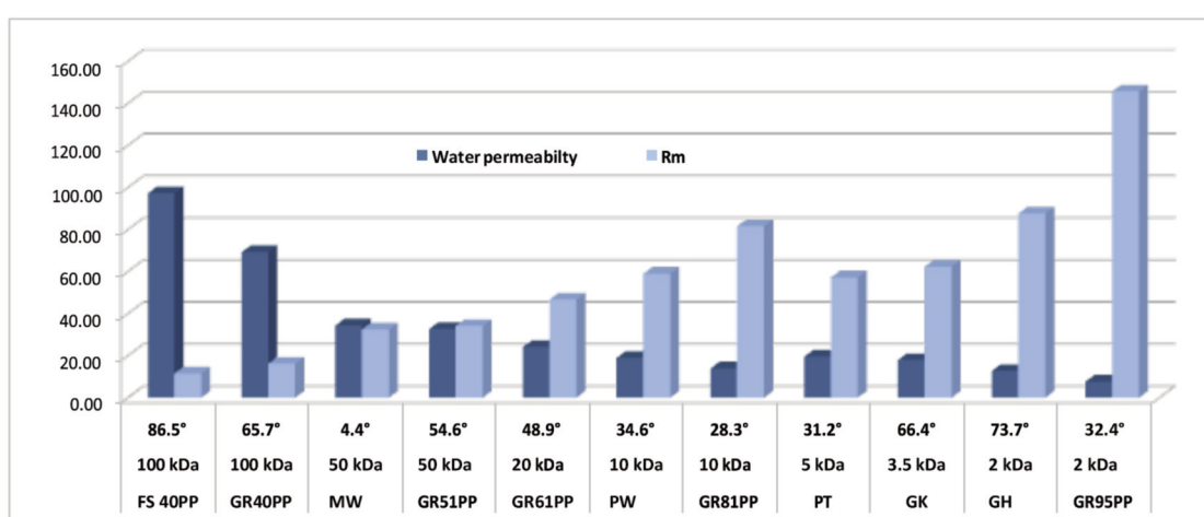
FIGURE 2. Hydraulic permeability ( Lm^{-2}h^{-1} \cdot 10^{-5} Pa ) and membrane resistance ( R_m ) 10 m^{-1} to water and contact angle for the ultrafiltration membranes ( T = 20 ^\circ C ).
