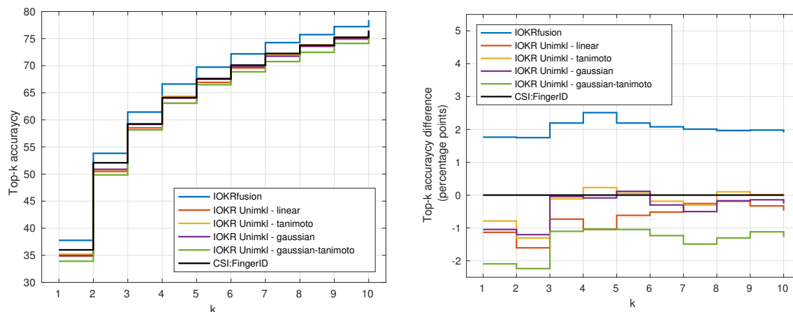
Figure 5. Plot of the top-k accuracy for IOKR Unimkl, CSI:FingerID and IOKRfusion in the positive ionization mode.
