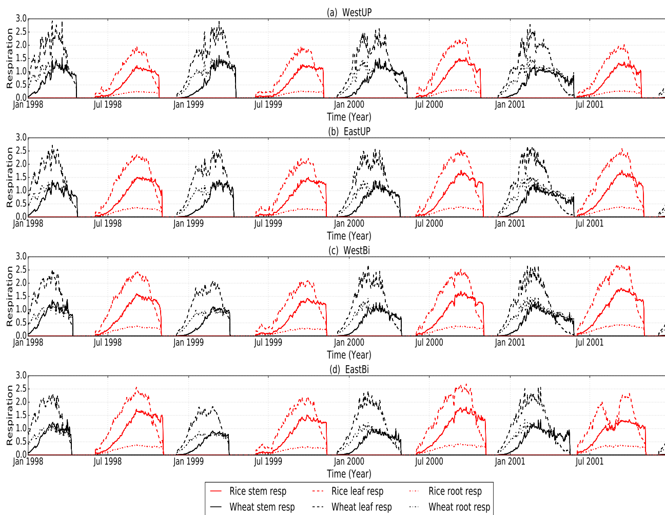
India point runs: Maintenance respiration for each crop ( gC\ m^{-2}\ day^{-1} )
