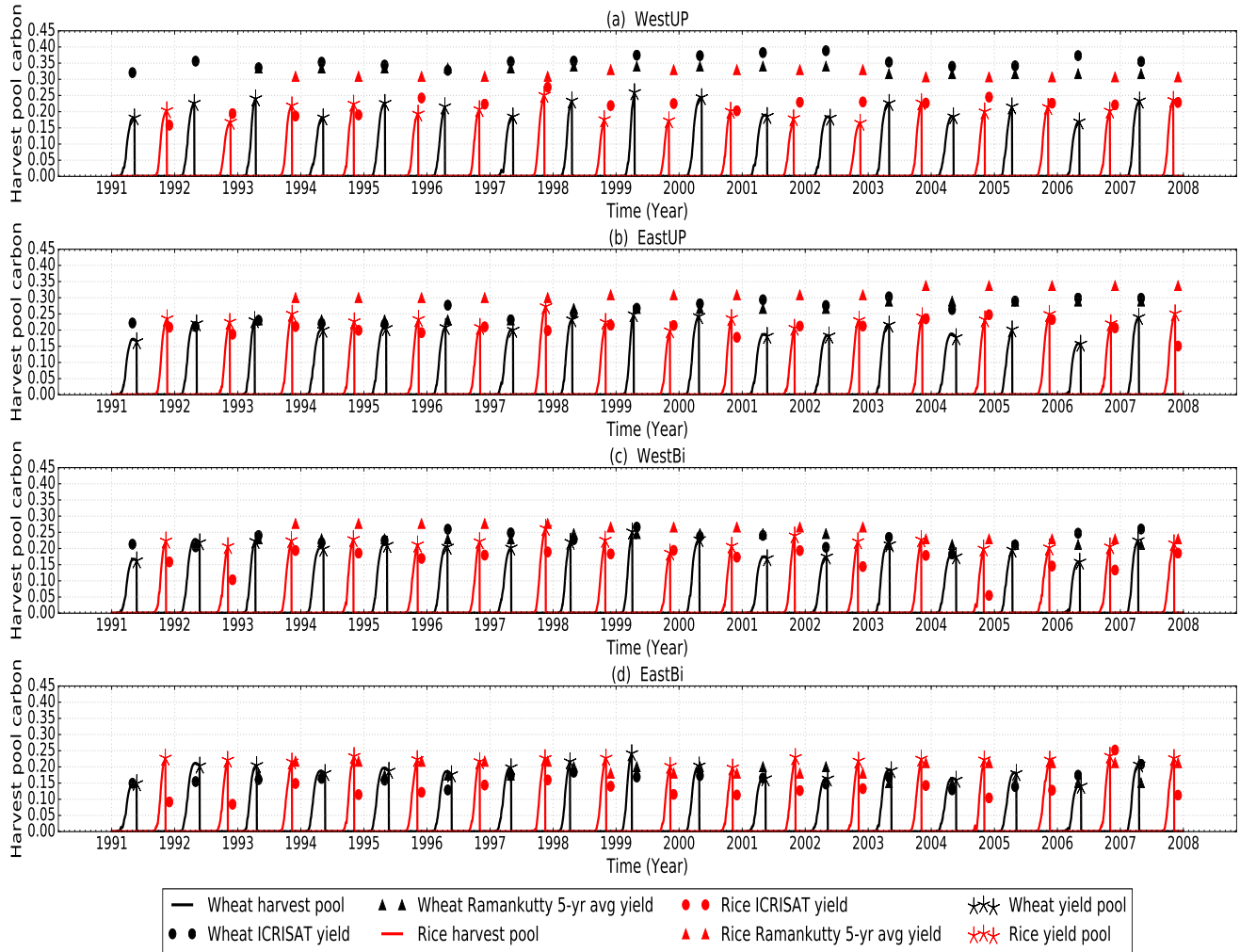
India point runs: Carbon in harvested parts of crop ( kg\ m^{-2} )
