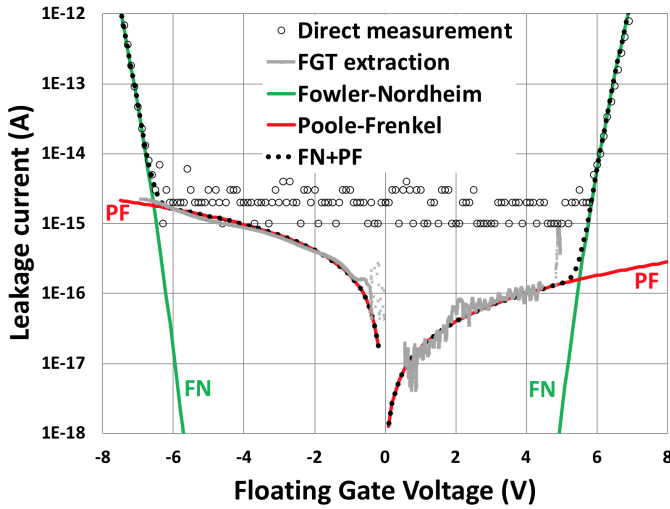
Figure 5. Modeling of both direct measurement and FGT extraction, using a combo of FN and PF mechanisms. \alpha_{FN} = 7.1 \times 10^{-4} A/V^2 , \beta_{FN} = 2.55 \times 10^{10} V/m , \alpha_{PF} = 1.26 \times 10^{-16} A/(V.m) , \beta_{FN} = 5 \times 10^{-7} (V.m)^{1/2}
