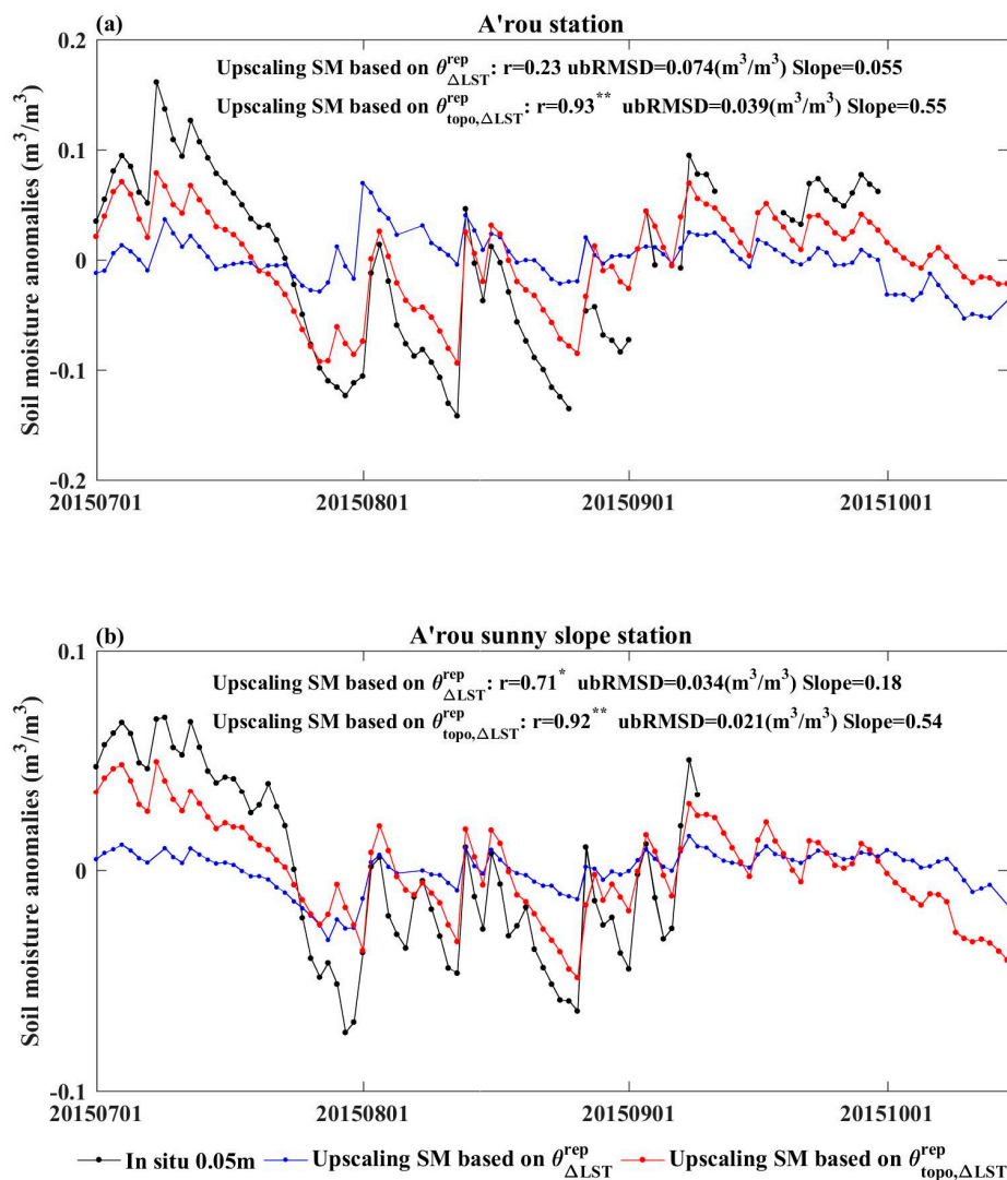
Figure 7. Time series of the upscaled SM based on \theta_{\Delta LST}^{rep} and \theta_{topo,\Delta LST}^{rep} against the in situ measured SM at the A'rou superstation (a) and the A'rou sunny (b) automatic meteorological stations. The ubRMSD values associated with the SM estimates and AMS observations were calculated by removing the mean values of the time series.
