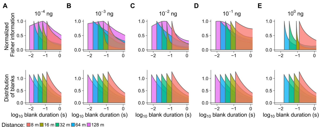
Fig 4. ORN coding precision of pheromone encounters is adjusted to the statistics of blanks in the plume. (Top row) Profiles of the coding accuracy (Fisher information) as a function of blank duration. The situation is shown for different pheromone doses (A–E) and virtual downwind distances from the source (color). Each Fisher information curve was individually scaled (normalized) to achieve that its maximum value is equal to 1. Stimulation by 10^0 ng pheromone dose was not performed for 128 m. (Bottom row) The distributions of blanks for the corresponding distances. With the exception of the largest distance (128 m), the Fisher information profiles follow the distribution profiles, which means that the coding resources are distributed in agreement with the frequency of various blank durations. In particular, the maximal coding accuracy, indicated by the location of the maximum Fisher information, tends to occur at the mode of the corresponding distribution, cf. Fig 5. The adjustment results in an average coding accuracy optimized for the particular distance (Fig 6).
