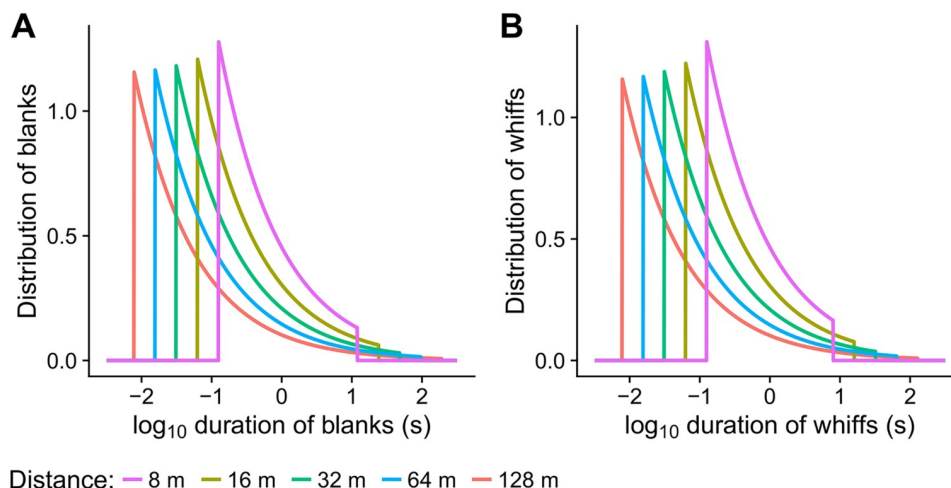
Fig 2. The temporal structure of the pheromone plume at a given downwind distance from the source (color) is characterized by the distribution of blanks and whiffs, which are independent. (A) Distribution of blanks, intervals without pheromone detection. (B) Distribution of whiffs, intervals with detectable pheromone presence.
