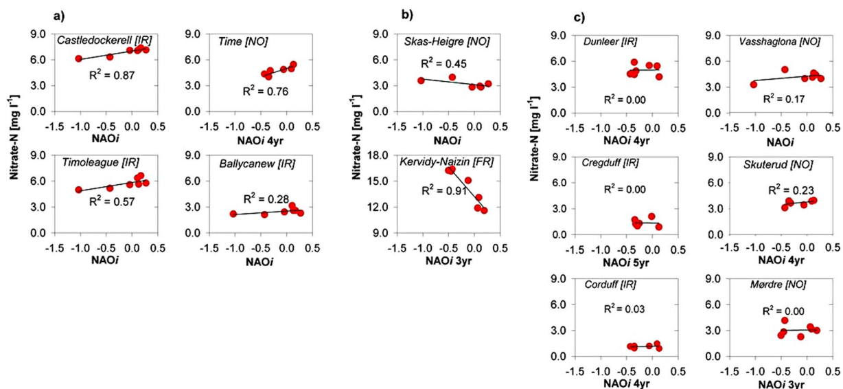
Figure 4. Linear correlation of nitrate-N concentrations in rivers to NAOi. Annual averages (hydrological years, October - September) of nitrate-N concentrations correlated to NAOi: (a) positive correlations, (b) negative correlations and (c) no correlations in Irish, Norwegian and French catchments with different flow controls, farm management, weather response to NAO change, N retention and storage capacity. NAOi are expressed as antecedent zero to five-year simple moving average depending on the specific catchment response time (there is no N concentration data for the Moulinet catchment).
