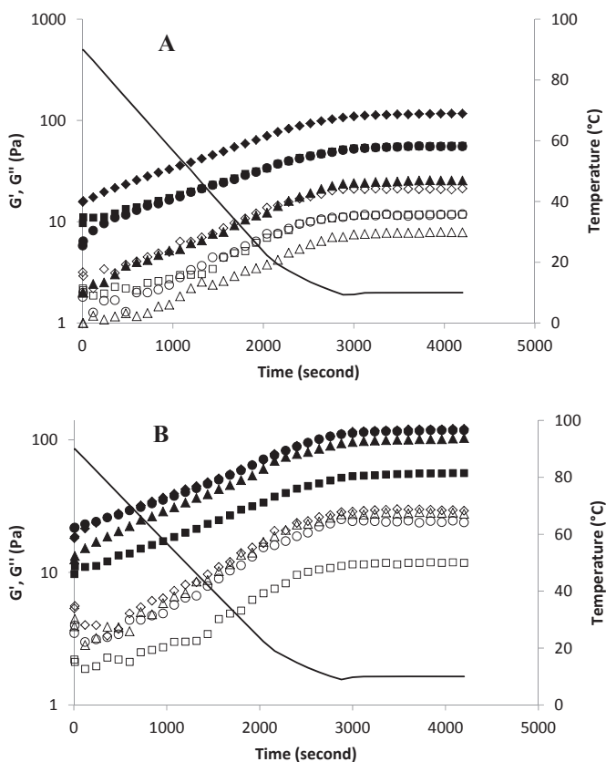
Fig. 4. Semi-logarithmic plots of G' and G'' vs time obtained at constant frequency (1 Hz) during controlled cooling ( 2\text{ }^{\circ}\text{C}/\text{min} ) of fibrous material gels. (A) Effect of the grinding time (To1, To3 and To6) and that of calcium (To3 and To3') on Tounsi fibrous material gelation. G' To6: ( \blacklozenge ), G'' To6: ( \diamond ), G' To1: ( \blacktriangle ) G'' To1: ( \Delta ), G' To3': ( \bullet ), G'' To3': ( \circ ), G' To3: ( \blacksquare ), G'' To3: ( \square ), Temperature: (-); (B) Rheological behaviour of fibrous material dispersions prepared from the four ecotypes after mechanical agitation (3 min) G' Ac: ( \blacklozenge ), G'' Ac: ( \diamond ), G' Ga: ( \blacktriangle ), G'' Ga: ( \Delta ), G' Ne: ( \bullet ), G'' Ne: ( \circ ), G' To: ( \blacksquare ), G'' To: ( \square ), Temperature: (-).
