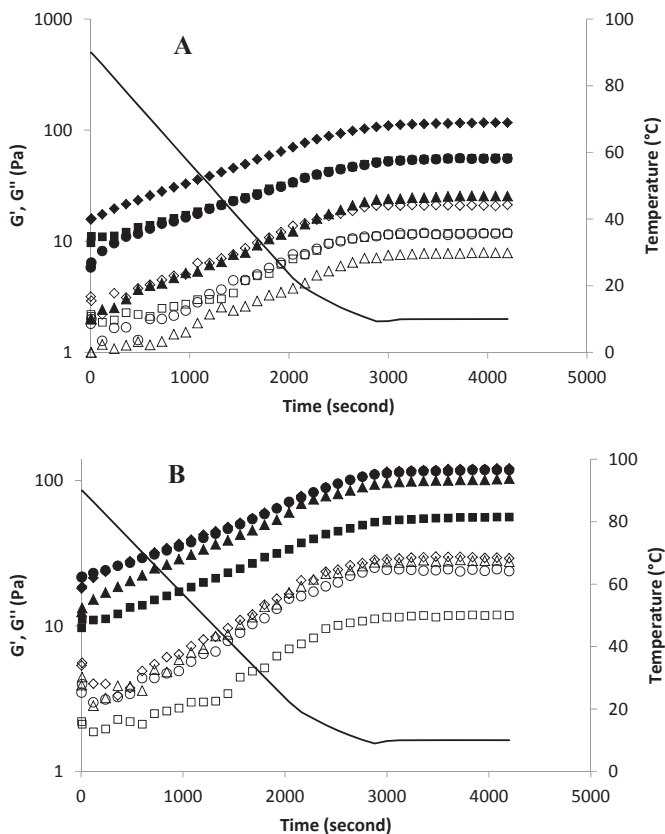
Fig. 4. Semi-logarithmic plots of G' and G'' vs time obtained at constant frequency (1 Hz) during controlled cooling (2 °C/min) of fibrous material gels. (A) Effect of the grinding time (To1, To3 and To6) and that of calcium (To3 and To3') on Tounsi fibrous material gelation. G' To6: (◆), G'' To6: (◇), G' To1: (▲), G'' To1: (Δ), G' To3': (●), G'' To3': (○), G' To3: (■), G'' To3: (□), Temperature: (-); (B) Rheological behaviour of fibrous material dispersions prepared from the four ecotypes after mechanical agitation (3 min) G' Ac: (◆), G'' Ac: (◇), G' Ga: (▲), G'' Ga: (Δ), G' Ne: (●), G'' Ne: (○), G' To: (■), G'' To: (□), Temperature: (-).
