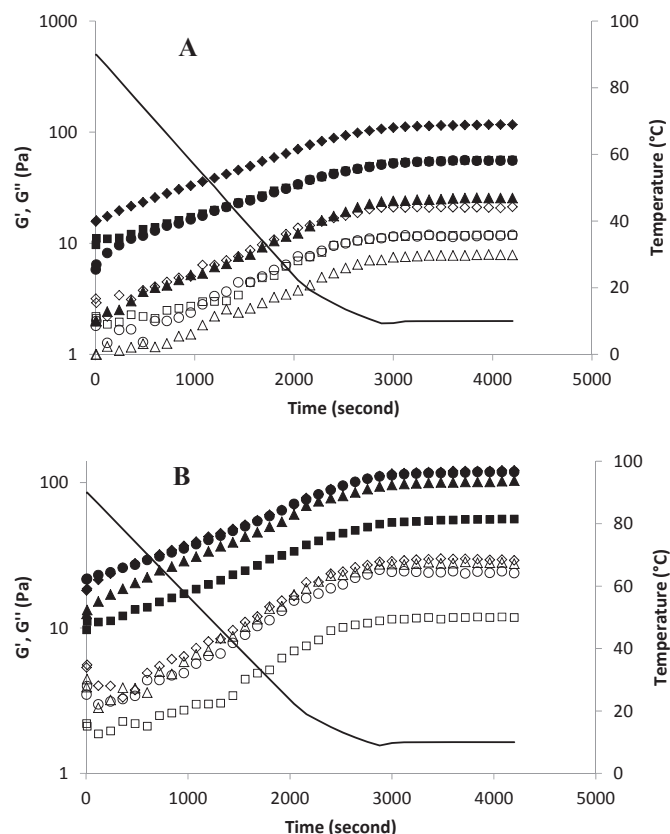
Fig. 4. Semi-logarithmic plots of G' and G'' vs time obtained at constant frequency (1 Hz) during controlled cooling (2 °C/min) of fibrous material gels. (A) Effect of the grinding time (To1, To3 and To6) and that of calcium (To3 and To3') on Tounsi fibrous material gelation. G' To6: (◆), G'' To6: (◇), G' To1: (▲), G'' To1: (Δ), G' To3: (●), G'' To3: (○), G' To3': (■), G'' To3': (□), Temperature: (-); (B) Rheological behaviour of fibrous material dispersions prepared from the four ecotypes after mechanical agitation (3 min) G' Ac: (◆), G'' Ac: (◇), G' Ga: (▲), G'' Ga: (Δ), G' Ne: (●), G'' Ne: (○), G' To: (■), G'' To: (□), Temperature: (-).
