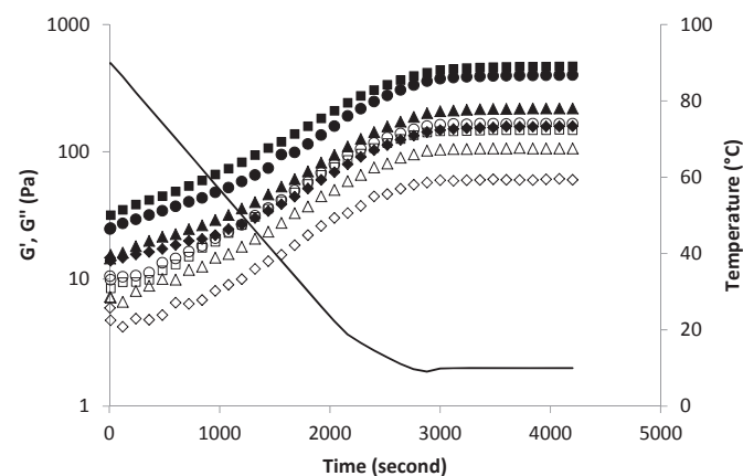
Fig. 1. Semi-logarithmic plots of G' and G'' vs time obtained at constant frequency (1 Hz) during controlled cooling (2 °C/min) of peel gels. G' Ac: (◆), G'' Ac: (◇), G' Ga: (▲), G'' Ga: (Δ), G' Ne: (●), G'' Ne: (○), G' To: (■), G'' To: (□), Temperature: (-).
