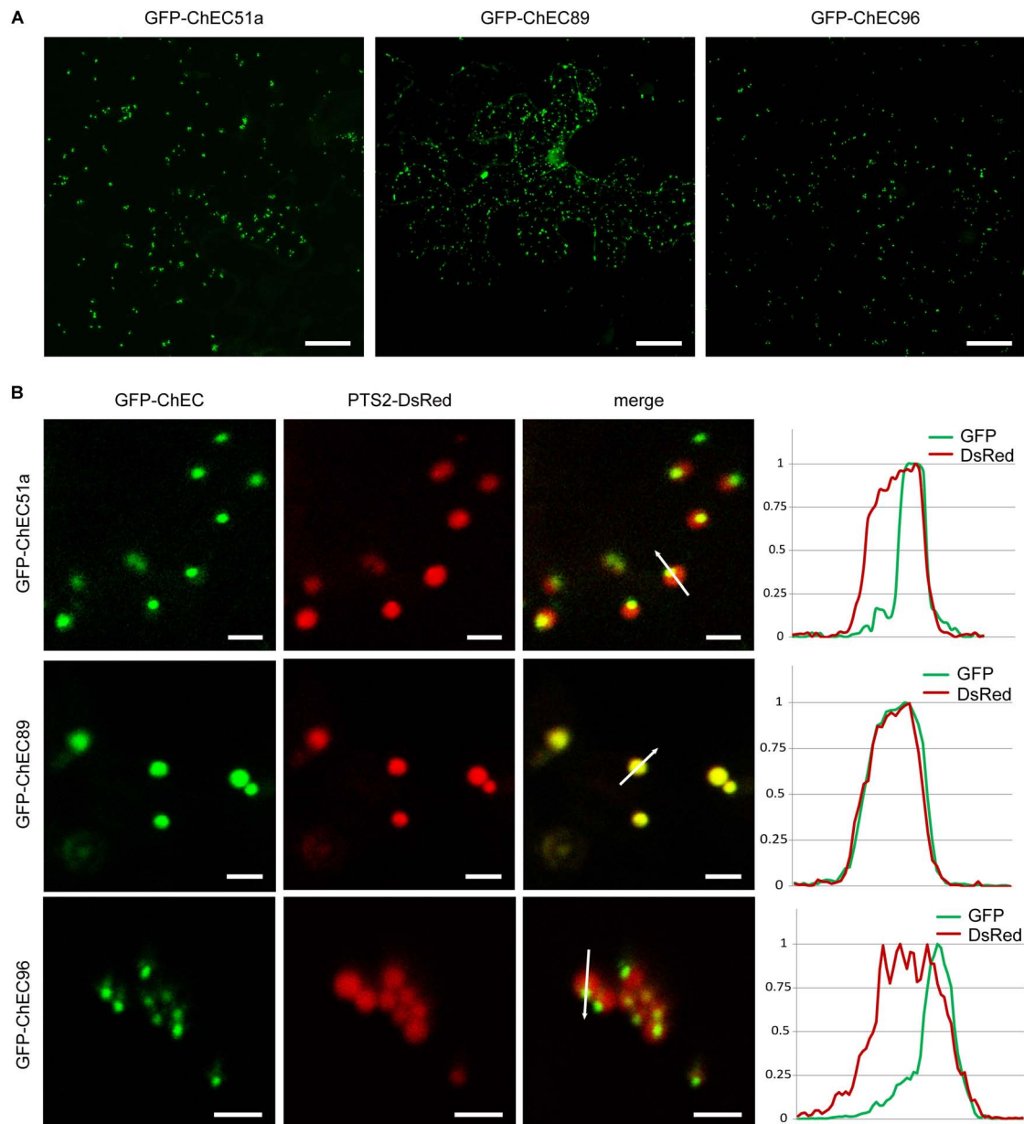
FIGURE 5 | GFP-tagged ChECs targeted to plant peroxisomes upon transient expression in N. benthamiana cells. (A) GFP-ChEC51a, GFP-ChEC89, and GFP-ChEC96 label small, highly mobile plant organelles. Bars = 25 \mu m. (B) All three fusion proteins co-localize with a PTS2-DsRed marker specific for plant peroxisomes. The right panels are fluorescence intensity plots across representative peroxisomes (white arrows) showing that while ChEC89 is distributed uniformly through the peroxisome matrix, ChEC51a and ChEC96 are concentrated in small punctate inclusions apparently located inside the matrix. Bars = 2.5 \mu m.
