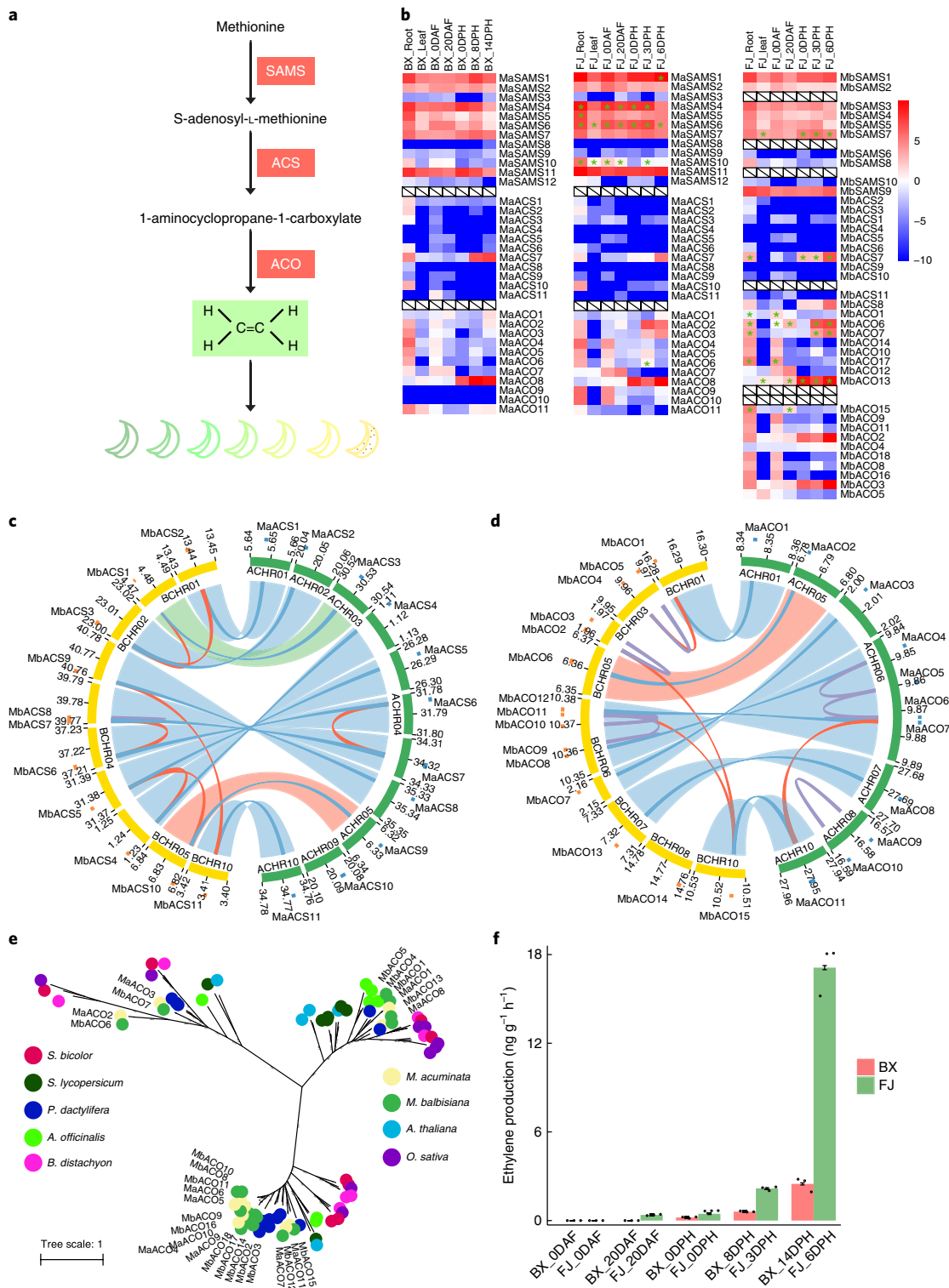
Fig. 3 | Phylogeny and expression patterns of ethylene biosynthesis genes between M. acuminata (A-genome) and M. balbisiana (B-genome). a , Overview of the ethylene biosynthesis pathway. b , Expression patterns of SAMS, ACS and ACO family genes in the root and leaf, and at different stages of fruit development and ripening in BX, the A-subgenome of FJ and the B-subgenome of FJ. Genes aligned horizontally in the heat map indicate homoeologue gene pairs between the A- and B-genomes. White boxes with diagonals indicate the lack of homoeologue gene pairs between the A- and B-subgenomes. Asterisks indicate expression dominance of homoeologue gene pairs between the A- and B-subgenomes of FJ. c,d , Synteny analysis of ACS ( c ) and ACO ( d ) families between the A- and B-genomes. Red lines indicate paralogous gene pairs resulting from WGD, blue lines indicate homoeologous gene pairs, purple lines indicate tandem duplication, light blue strips indicate aligned syntenic blocks, light green strip indicates translocation block and light red strips indicate inversion blocks. The blocks in outer ring represent location and length of genes; blue blocks represent genes from A-genome and orange blocks represent genes from B-genome. e , Phylogenetic analysis of ACO family genes among nine species: M. acuminata , M. balbisiana , A. thaliana , O. sativa , Sorghum bicolor , Solanum lycopersicum , Phoenix dactylifera , Asparagus officinalis and B. distachyon . f , Ethylene production at different stages of fruit development and ripening in BX and FJ. Error bars show standard error of the mean from three independent experiments ( n=3 ).
