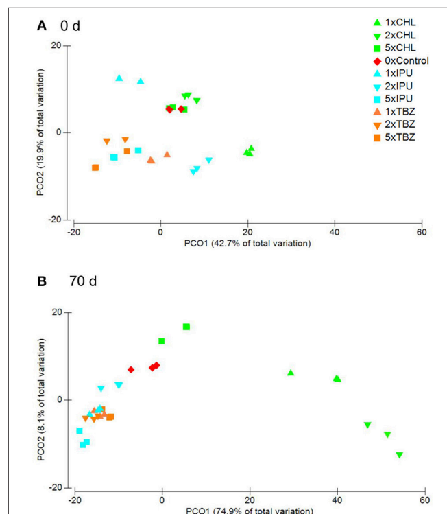
FIGURE 1 | Field study—PcoA on Bray Curtis similarity matrices based on presence and absence of bacterial OTUs in controls (0x dose) and samples treated with CHL, IPU, or TBZ (1, 2x or 5x recommended agronomical doses) and collected at (A) 0 days or (B) 70 days after treatment. For each treatment values of each of the three replicates are shown. Variance is expressed in % on each axis.
