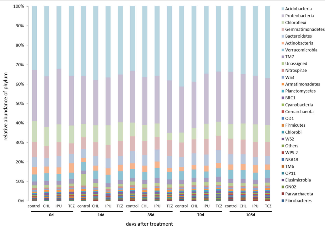
FIGURE 3 | Field study—The relative abundance (%) of bacterial phyla in the untreated (control) and pesticide-treated (CHL, IPU, or TCZ at 5x dose) soil samples at different time points (0, 14, 35, 70, and 105 days after treatment). Bacterial phyla whose abundance sum of all samples was <0.05% were grouped as “others.” 16S rDNA sequences that could not be assigned to a phylum were grouped as “unassigned”.
