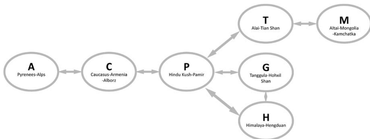
Figure 3. Diagram representing a corridor model, encompassing a set of the short-distance dispersal events permitted (in either direction) between the areas defined in Table 1, based on their geographical proximity and the likely disposition of suitable habitat within mountain ranges and favourable climates in the past (see the text).
