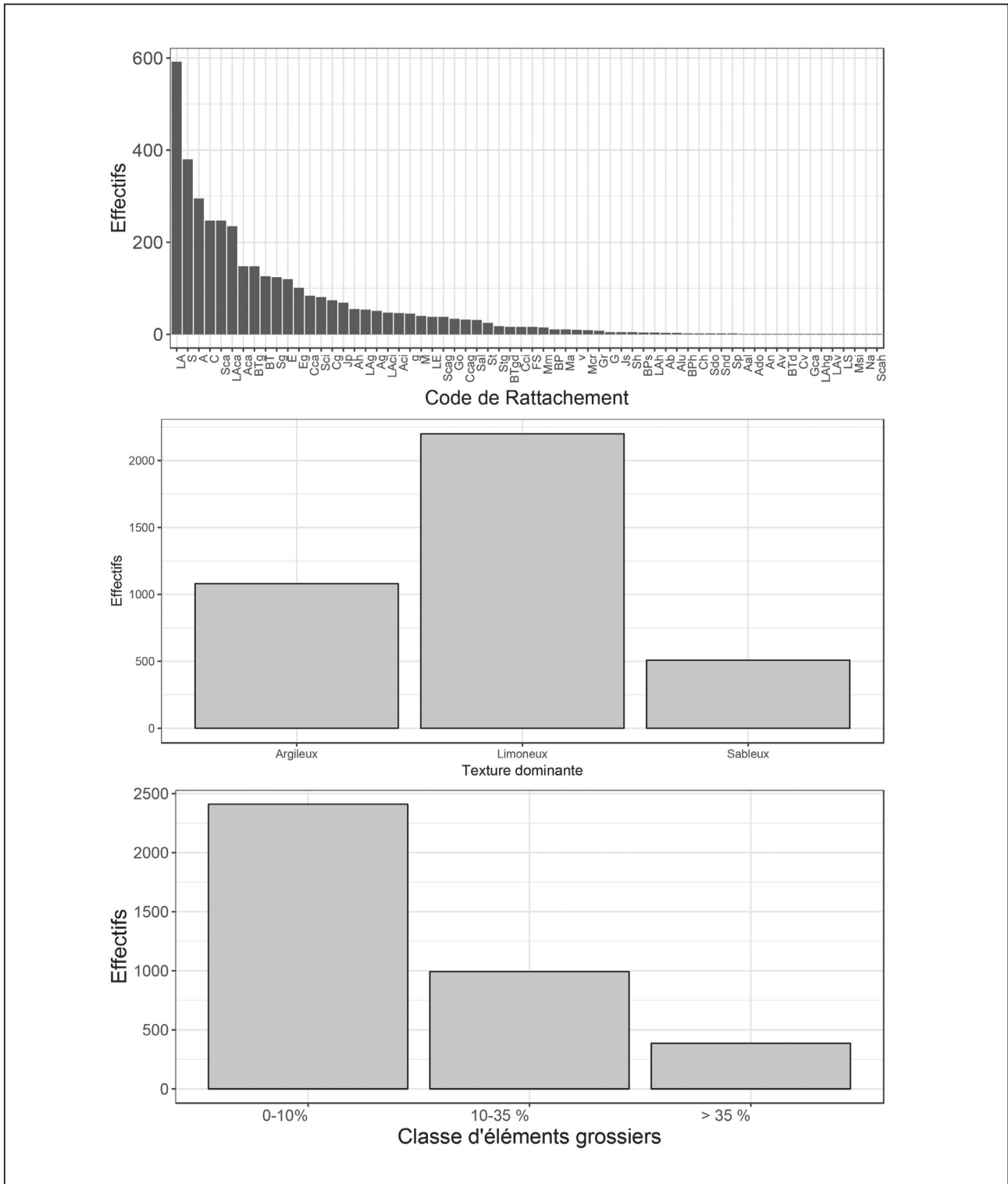
Figure2 - distribution of the horizon types, the dominant texture class and the amount of coarse fragments among the selected list of horizon types for selected for a measurement of AWC during the second RMQS campaign.
