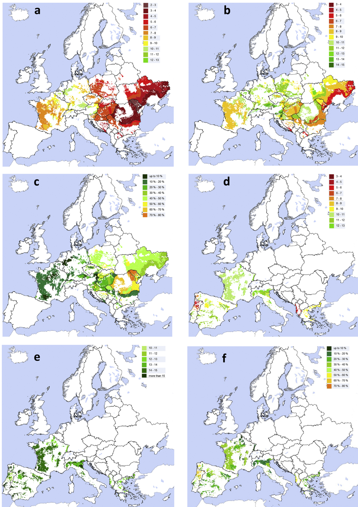
Fig. 2. Average crop yields ( t\ ha^{-1} at standard moisture content) and yield gaps (% of yield potential) of rainfed maize (a,b,c) and irrigated maize (d,e,f) for climate zones in countries. Actual yield (a,d), water-limited yield (b), potential yield (e) and yield gap (c,f). Crop area mask of You et al. (2014).
