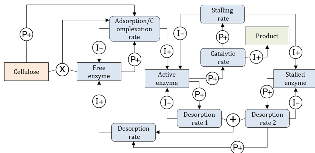
Figure 9. Qualitative Reasoning Model M2 for stalling of enzyme. Relationship with the numerical model (Eq. 3) is given in Table 5. Orange denotes substrate-related quantities, blue-grey is used for enzyme related quantities, and green denotes product related quantities.
